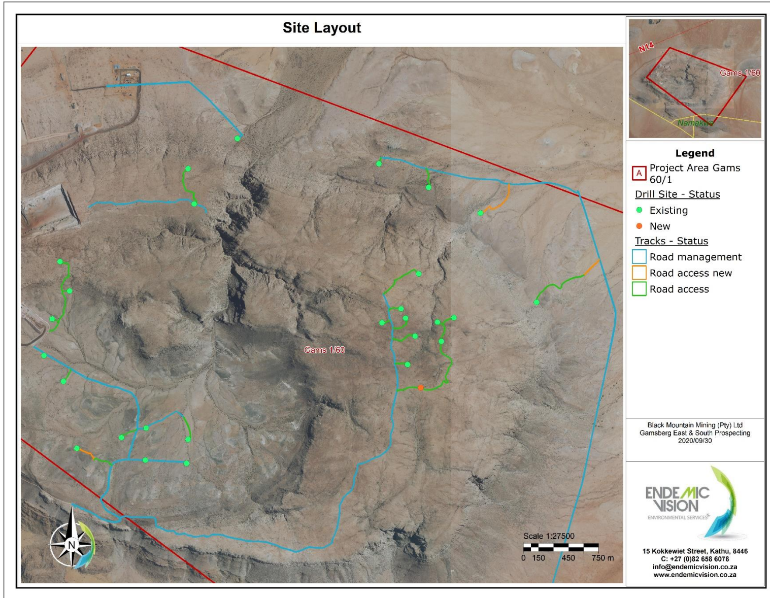
FIGURE 3: PLANNED SITE LAYOUT PLAN
