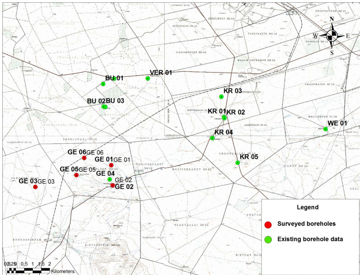
Figure 6: Hydrocensus results
