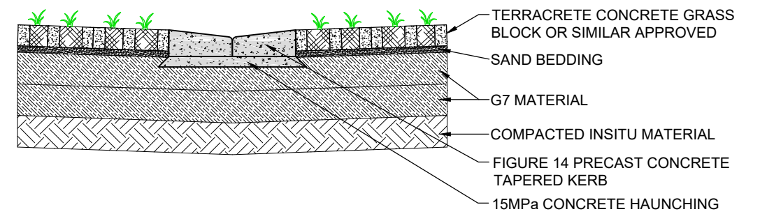
TYPICAL PARKING BAY SECTION B-B
