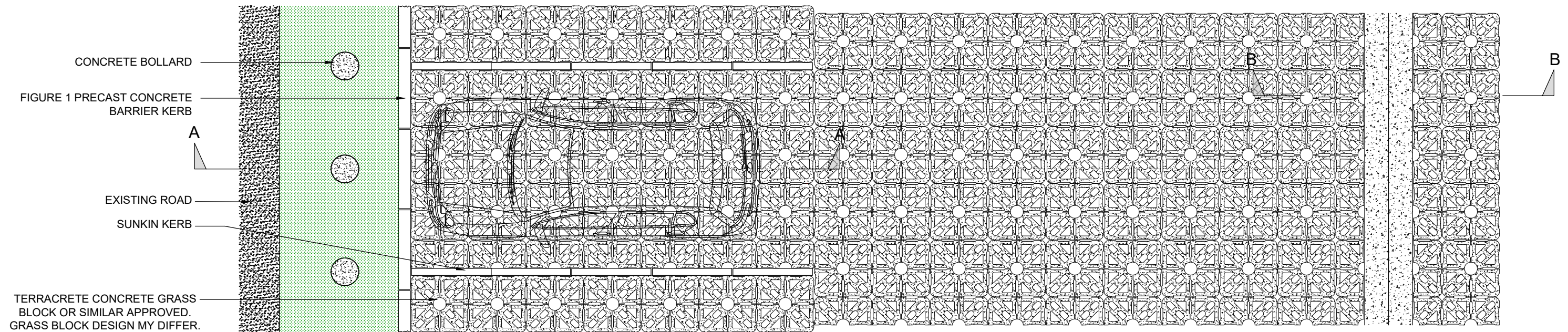
TYPICAL PARKING BAY PLAN
