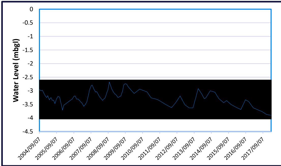
Figure 2-4: Groundwater level fluctuation in Monitoring Borehole DWA G1N0389 on the study site
