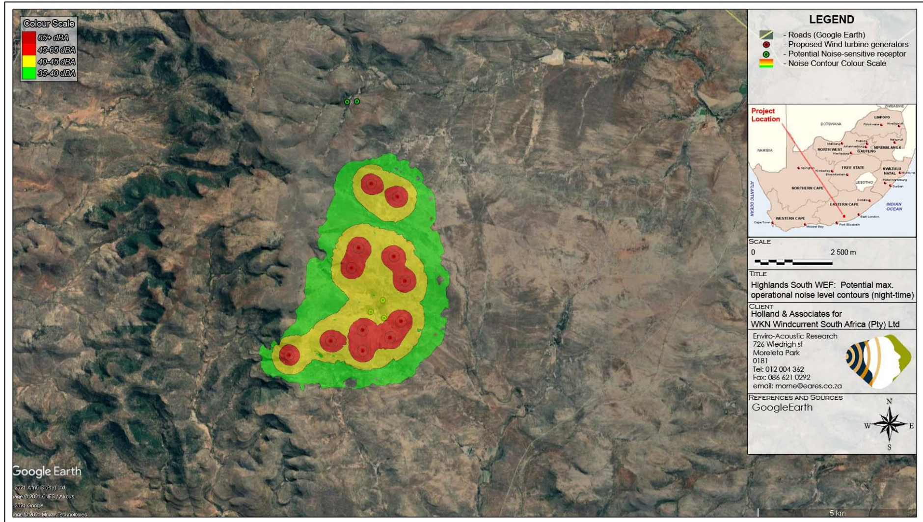
Figure 8-3: Projected maximum night-time operational noise rating levels due to operation of Highlands South WEF: Proposed amended layout
