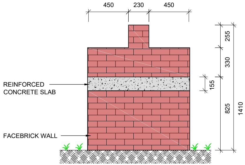
TYPICAL 4 x BRAAI ELEVATION 2
