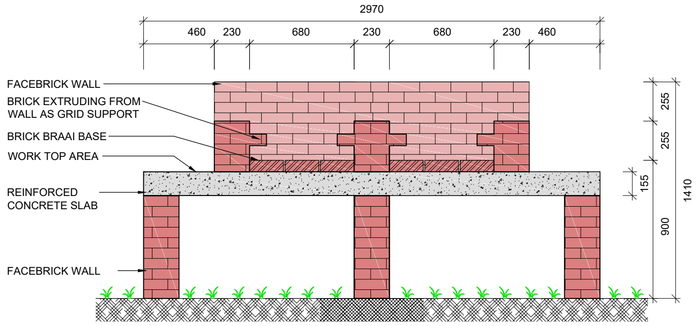
TYPICAL 4 x BRAAI ELEVATION 1
