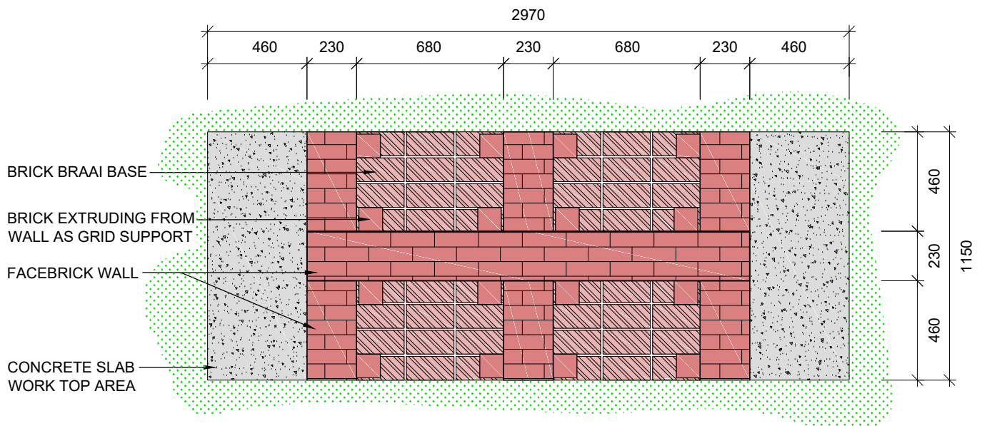
TYPICAL 4 x BRAAI PLAN
