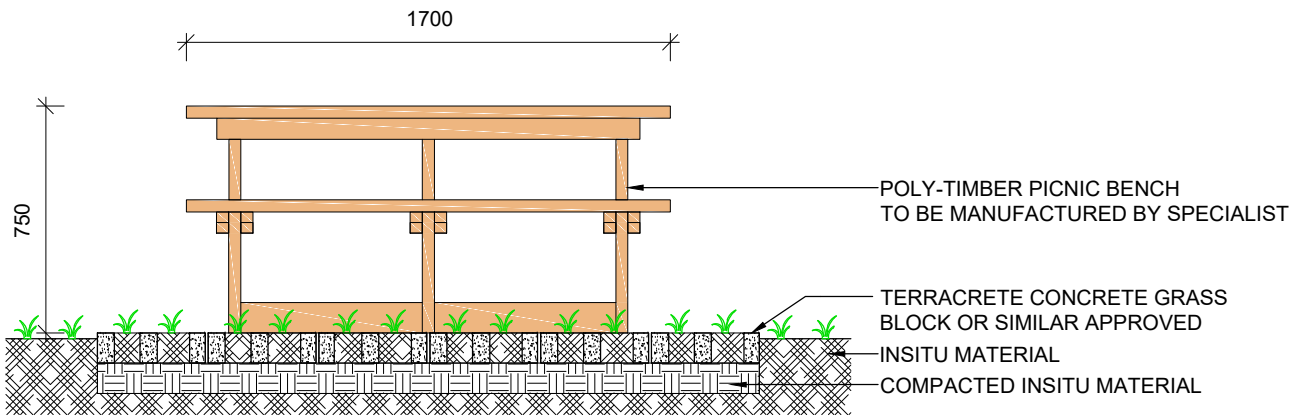
TYPICAL PICNIC BENCH ELEVATION 1
