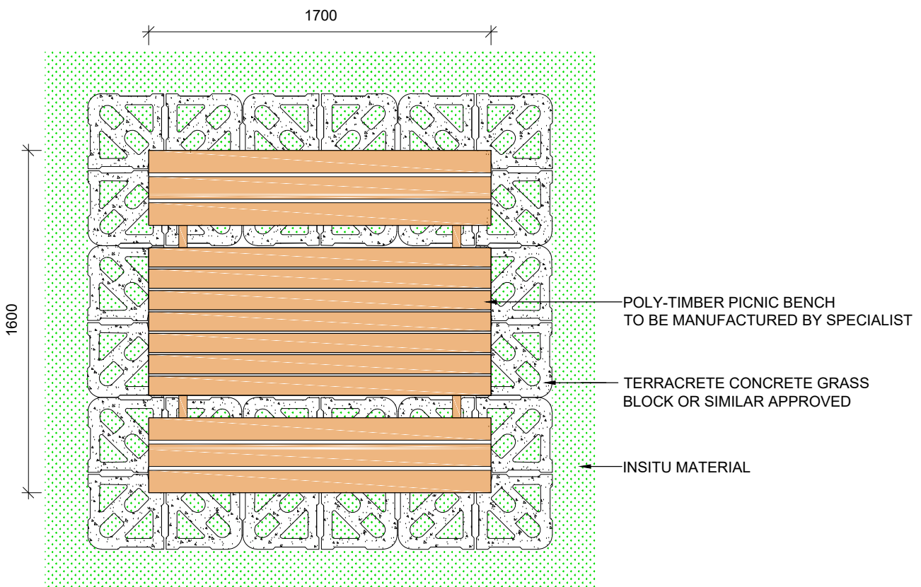
TYPICAL PICNIC BENCH PLAN
