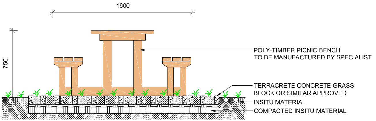
TYPICAL PICNIC BENCH ELEVATION 2
