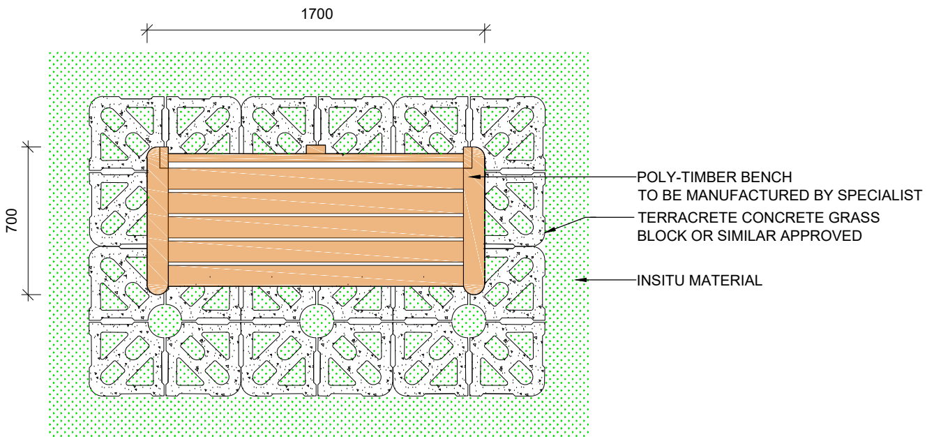
TYPICAL BENCH PLAN
