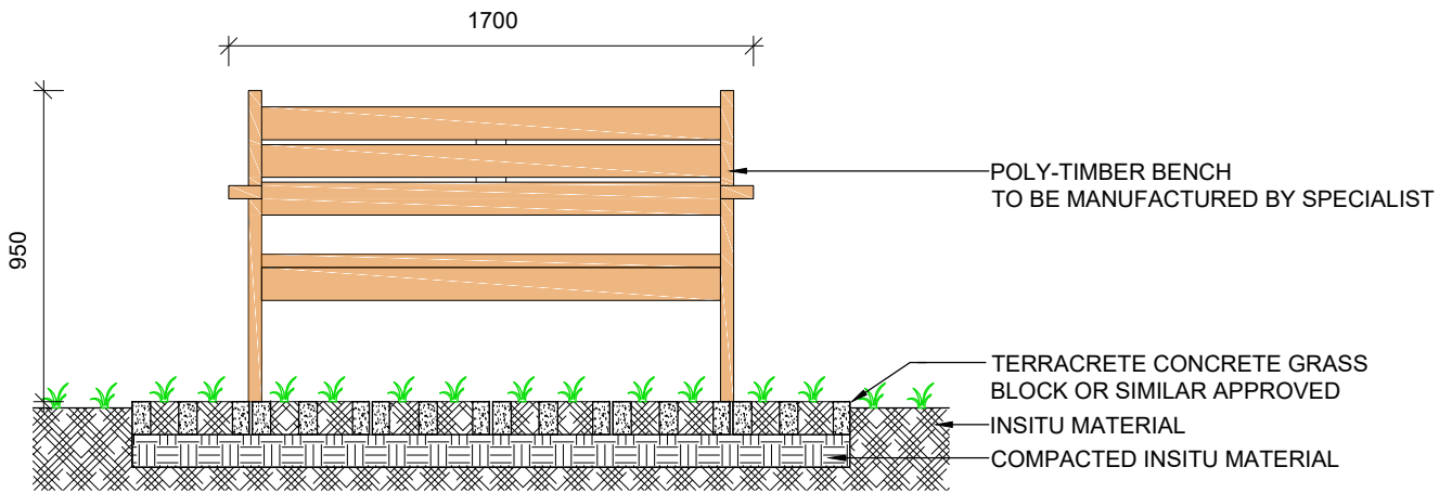
TYPICAL BENCH ELEVATION 1
