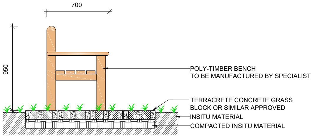
TYPICAL BENCH ELEVATION 2
