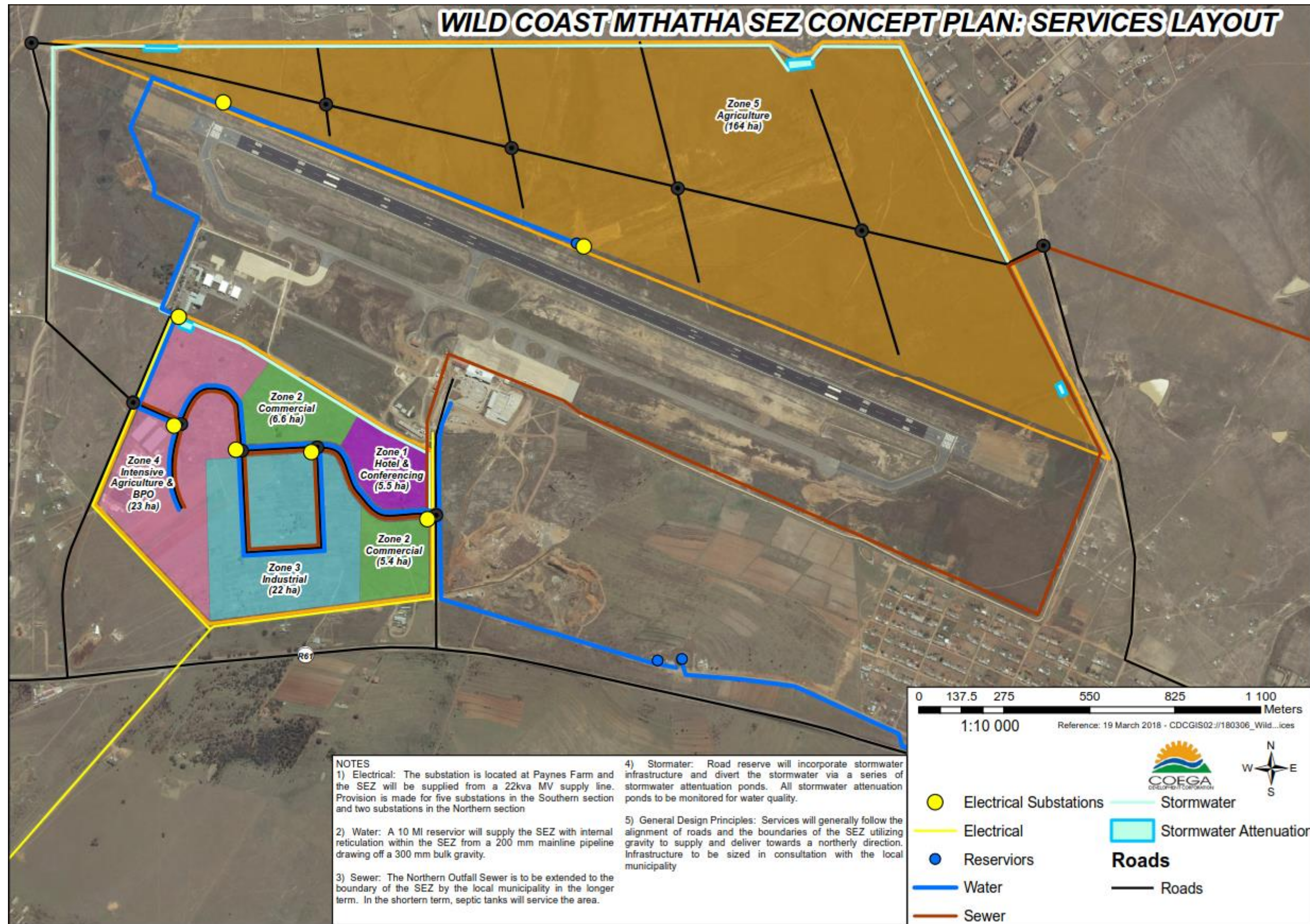
Figure 1: Site Layout
