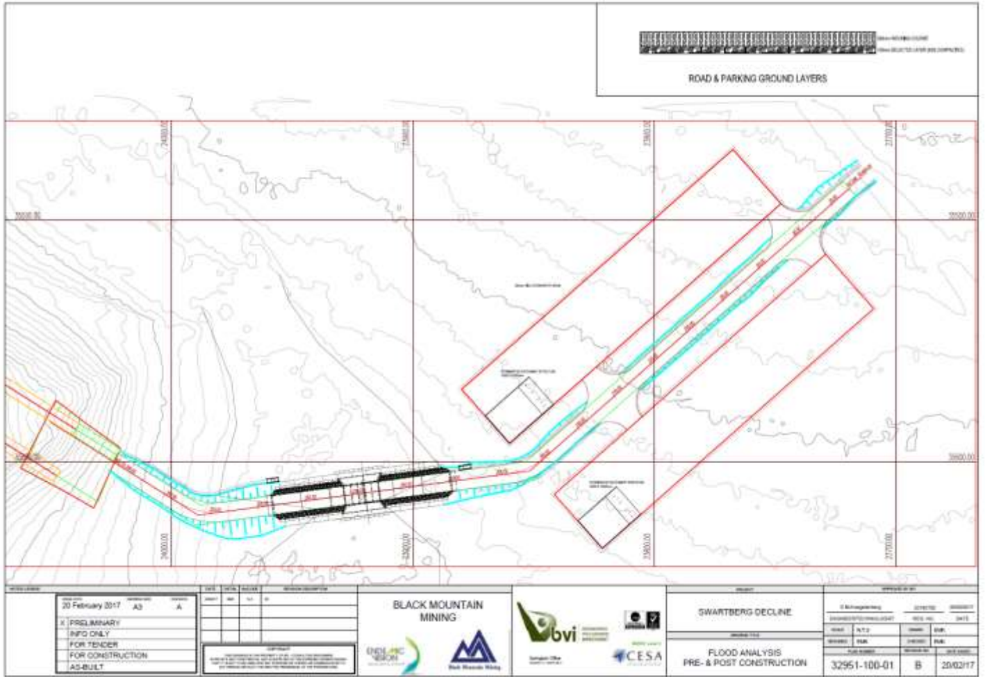
Figure 2: Final Design and storm water works
