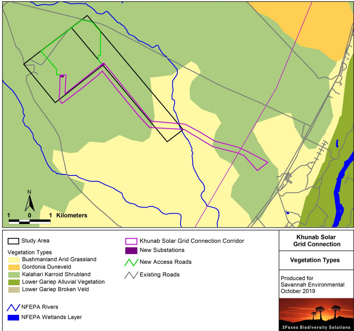
Figure 7. Broad-scale overview of the vegetation in and around the Khunab Solar Grid Connection. The vegetation map is an extract of the national vegetation map (Mucina & Rutherford 2006 & 2016 update) and also includes drainage lines delineated by the NFEPA assessment (Nel et al. 2011).
