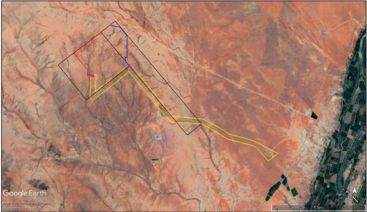
Figure 1. Locality map of the grid connection corridor showing the layout of the grid connection corridor.
