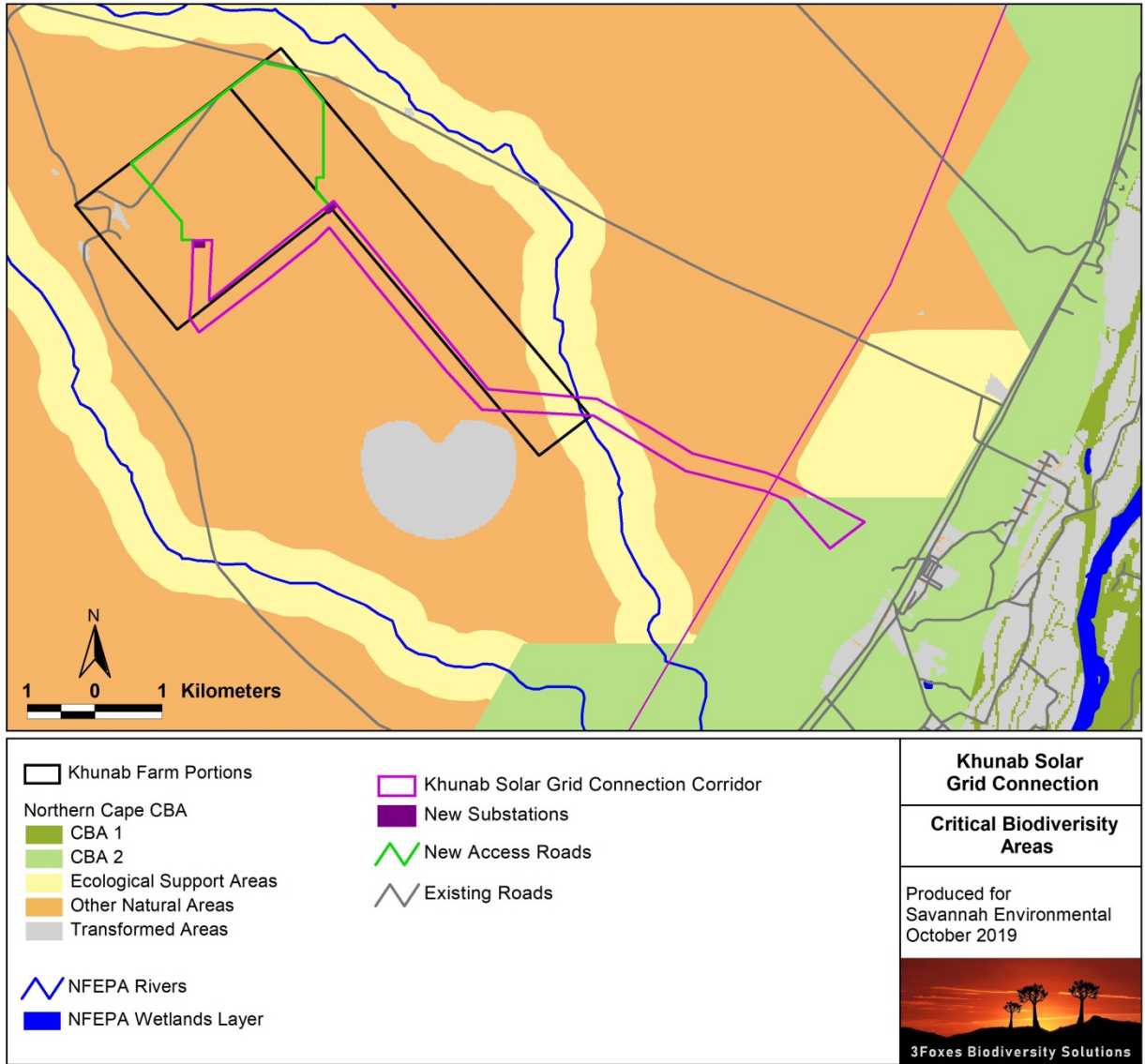
Figure 8. Extract of the Northern Cape Critical Biodiversity Areas map for the broader study area, showing that it is only the area around the existing Upington MTS that is a CBA2 and the rest of the development area identified for the establishment of the Khunab Solar Grid Connection would not impact any other CBAs.
