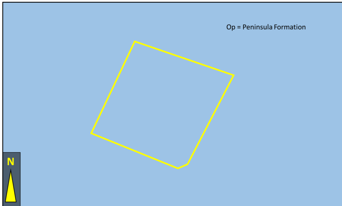
Figure 3 Geologic map underlying the study area in the Eastern Cape. proposed Solar Development on ERF 77 marked in yellow. (Op) Peninsula.
