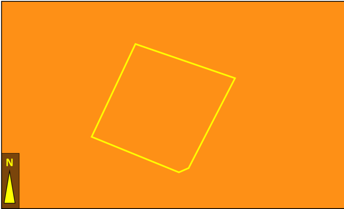
Figure 2 Palaeo-sensitivity Map. Adapted from https://sahris.sahra.org.za/map/palaeo . Indicating high fossil sensitivity underlying the study area in the Eastern Cape. Solar development marked in yellow within the orange zonation.
