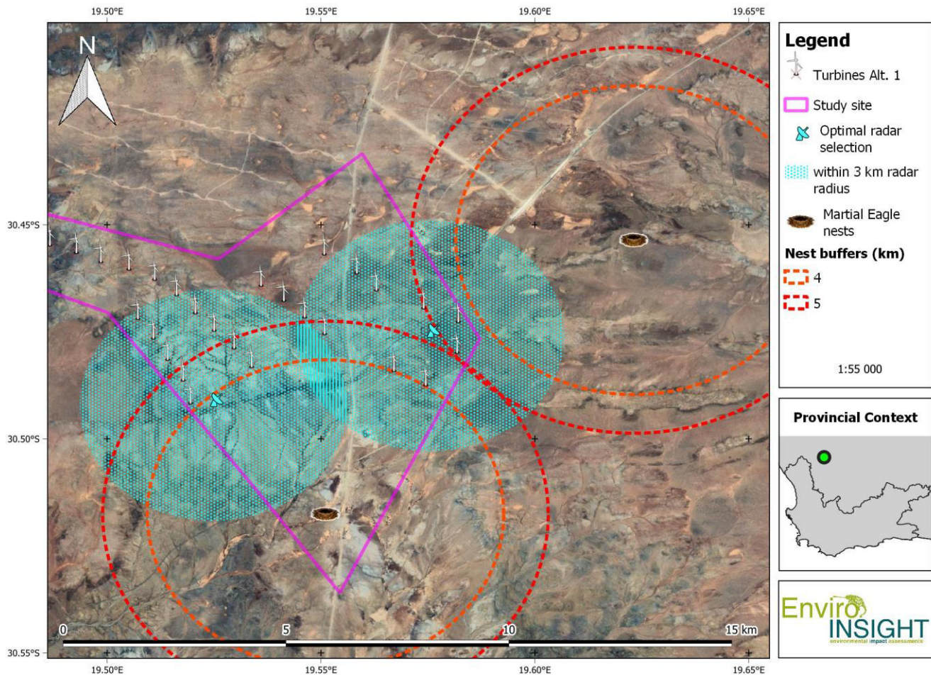
Figure 5-6: Final recommended placement of radar for shutdown on demand protocols
