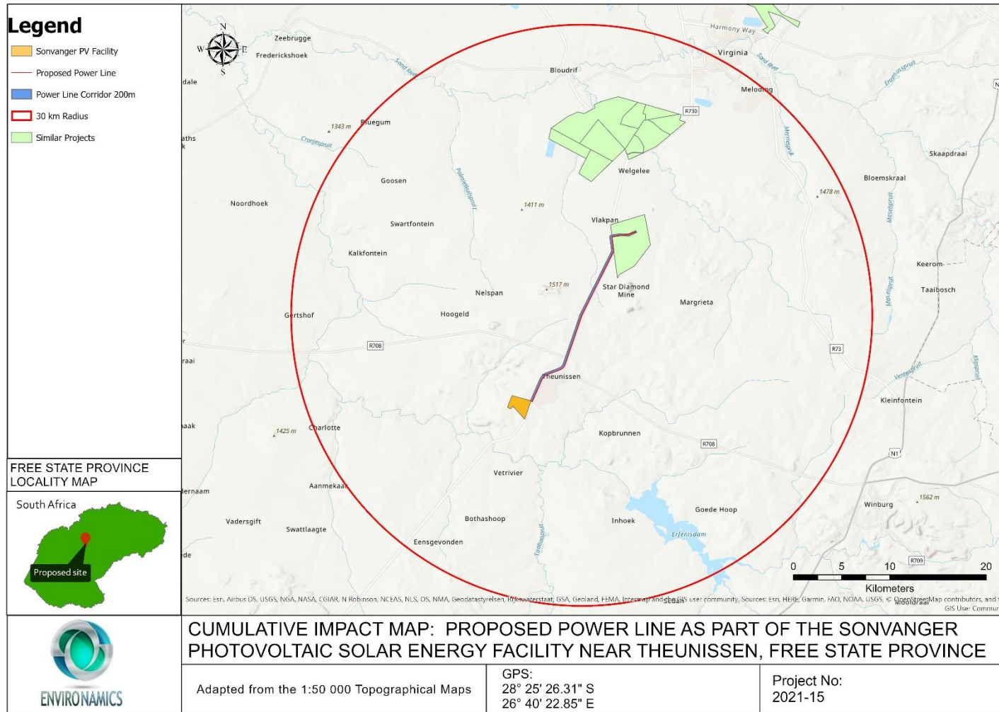
Figure 10. Cumulative impact map of the proposed powerline development in combination with other renewable energy developments in a 30 kilometer radius
