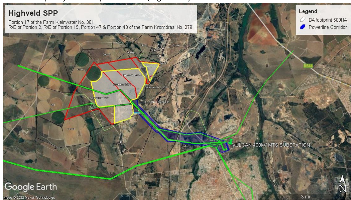
Figure 1-1 Powerline corridor
