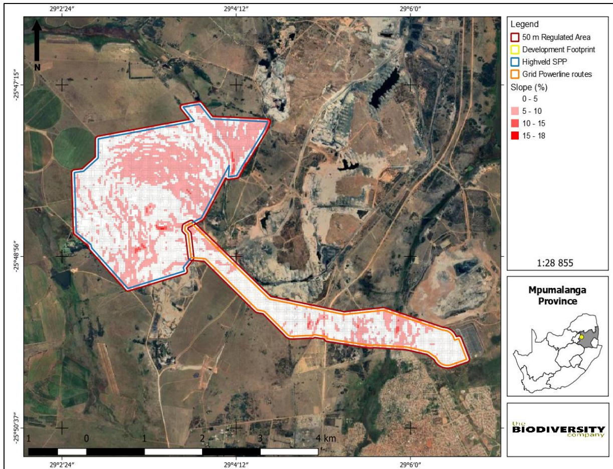
Figure 4-4 The slope percentage calculated for the project area
