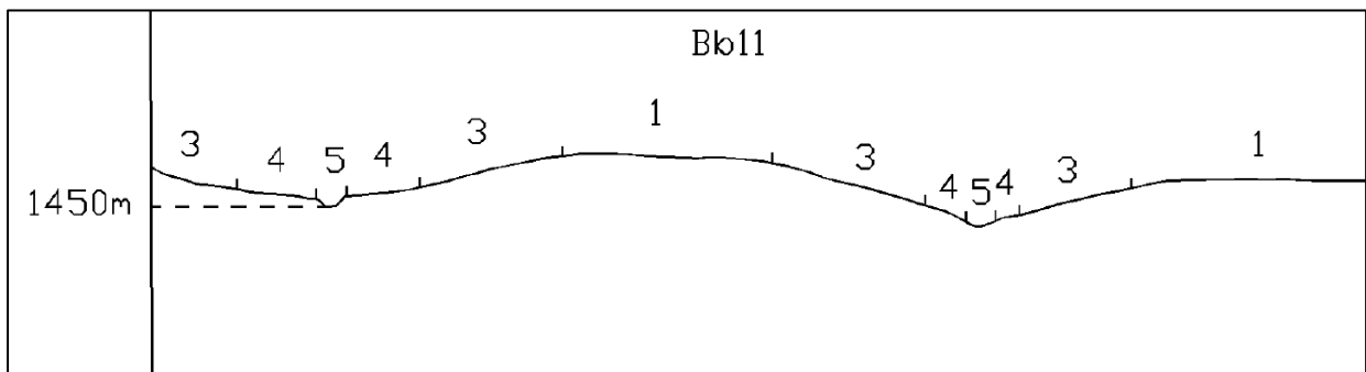
Figure 4-1 Illustration of land type Bb 11 terrain unit (Land Type Survey Staff, 1972 - 2006)
