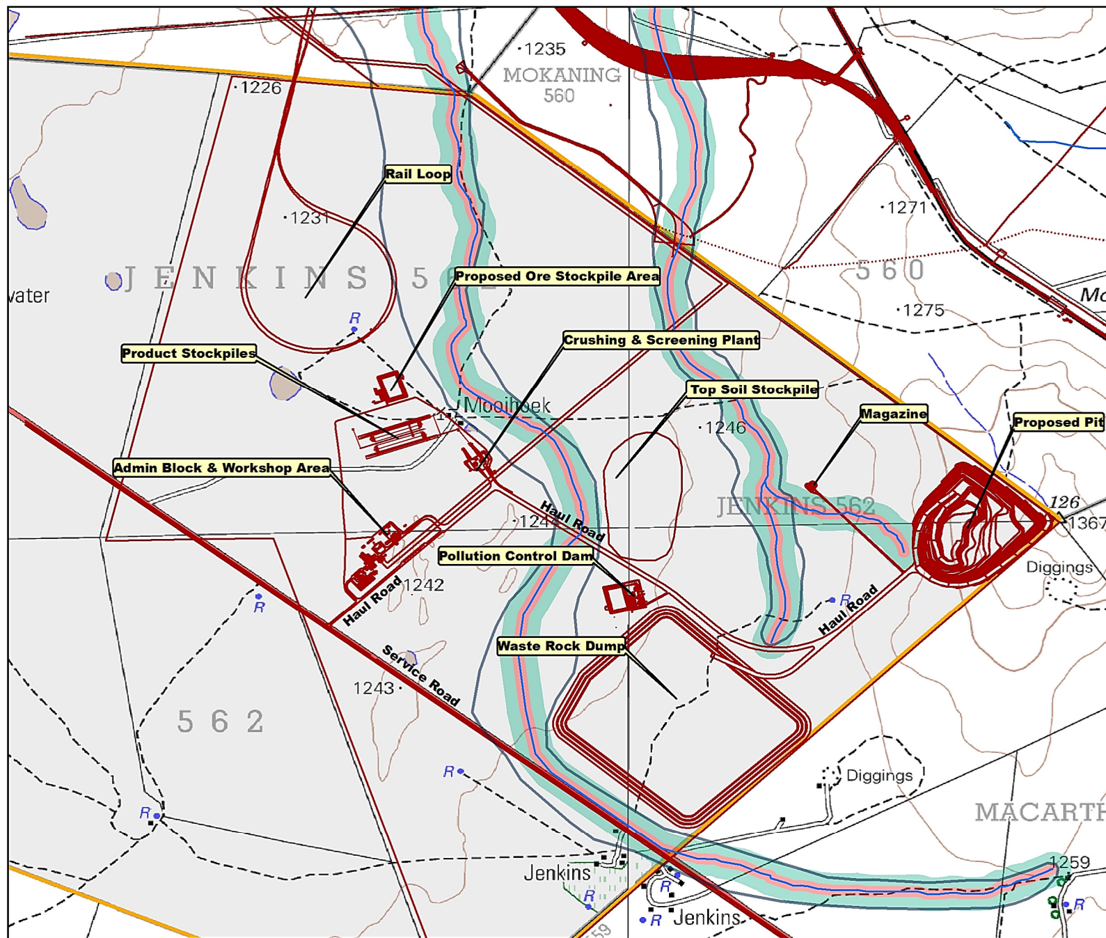
Figure 3: Infrastructure Plan
