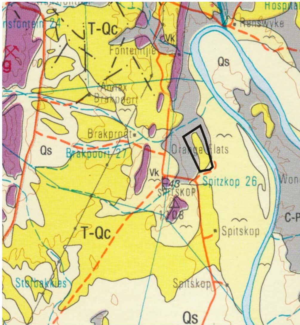
Figure 3. According to the 1:250 000 scale geological map 2922 Prieska, the study area is primarily underlain by localized outcrops of the Karoo Supergroup, Mbizane Formation (C-pd), covered by variable clasts of surface gravels, limestones (T-Qc), Quaternary aeolian sands (Qs) and sandy soils.
