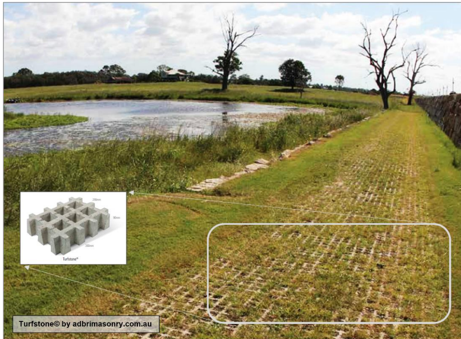
Figure 7-4 Example of permeable paving for roads and habitat maintenance
