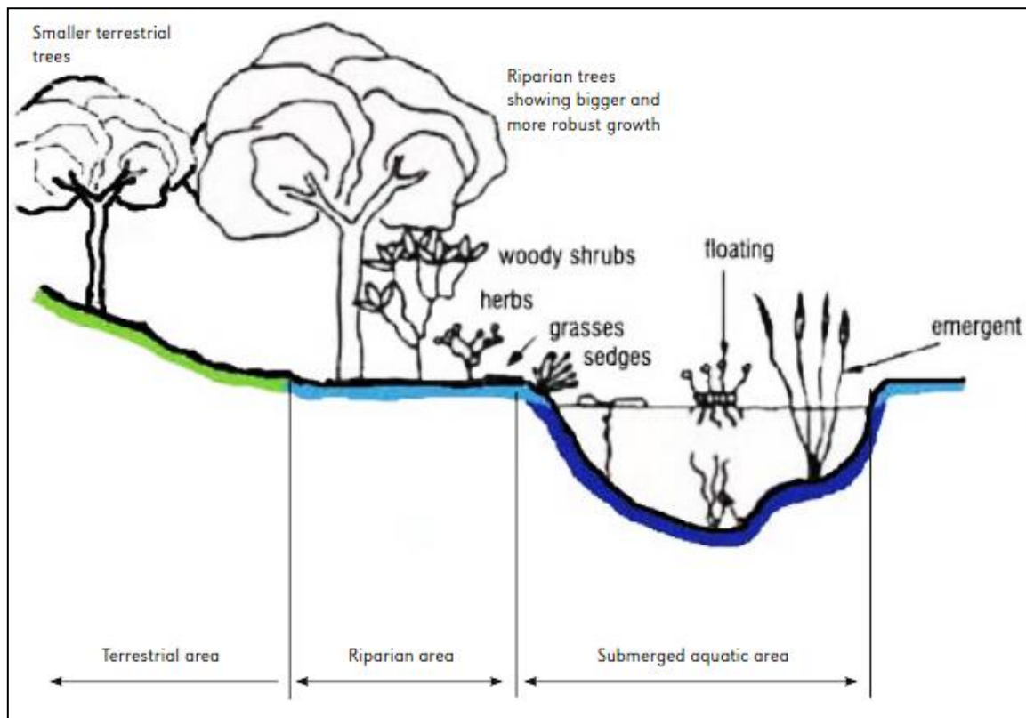
Figure 4-1 Riparian Habitat Delineations (DAAF, 2005)
