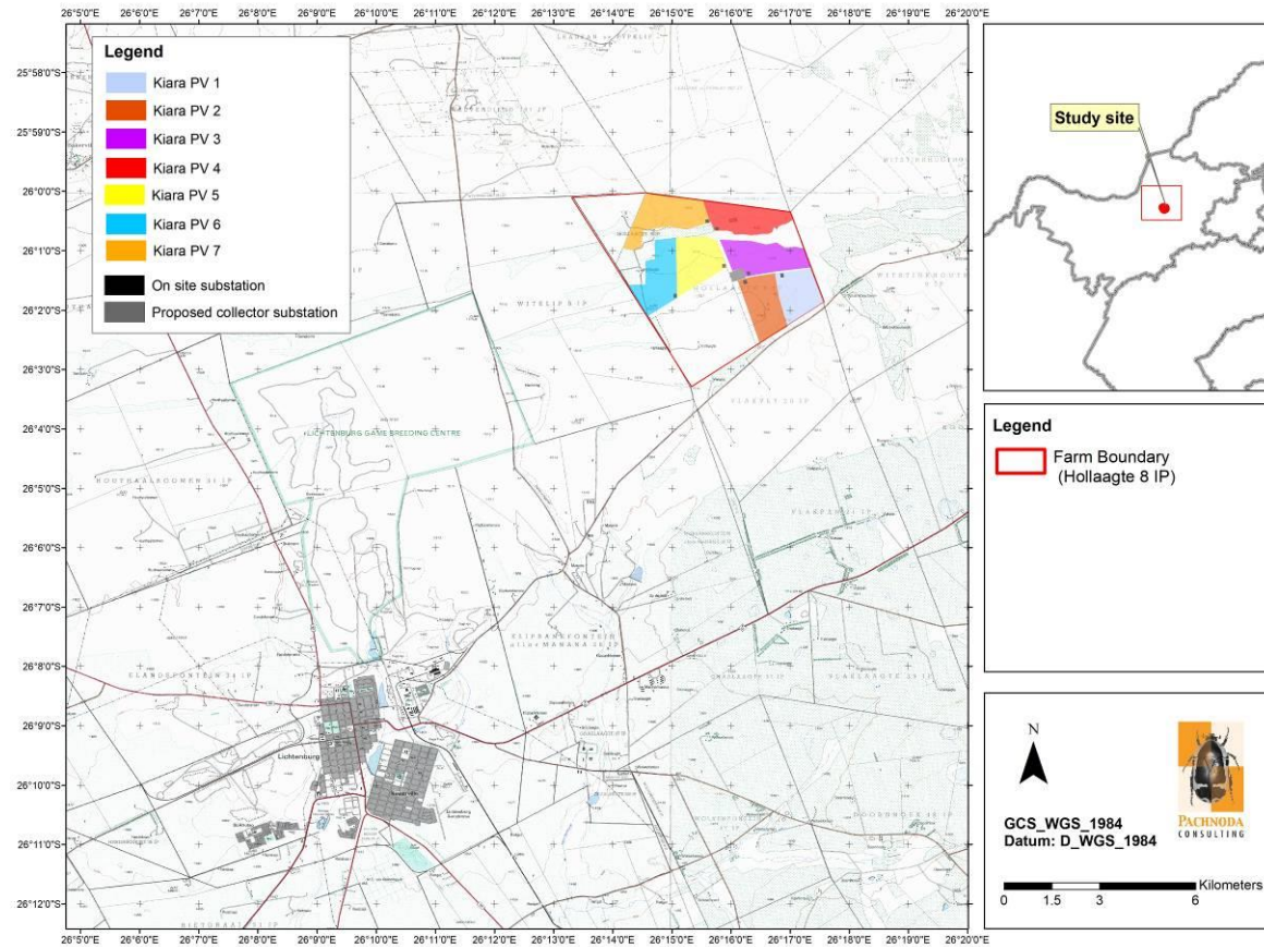
Figure 1: An ortho-cadastral map illustrating the geographic position of the proposed Kiara PV 4 facility in relation to six other planned PV facilities corresponding to the Farm Hollaagte No. 8.
