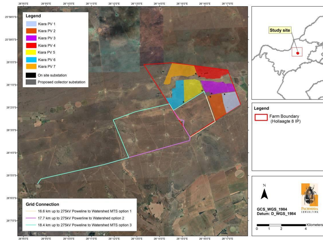
Figure 2: A satellite image illustrating the geographic position of the proposed Kiara PV 4 facility in relation to six other planned PV facilities corresponding and the proposed grid connection options.
