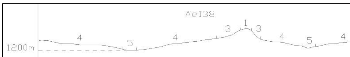
Figure 2-5 Illustration of the Ae 138 land type terrain units (Land Type Survey Staff, 1972 - 2006)
