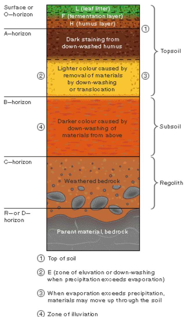
Figure 3. Soil system with different layers.
