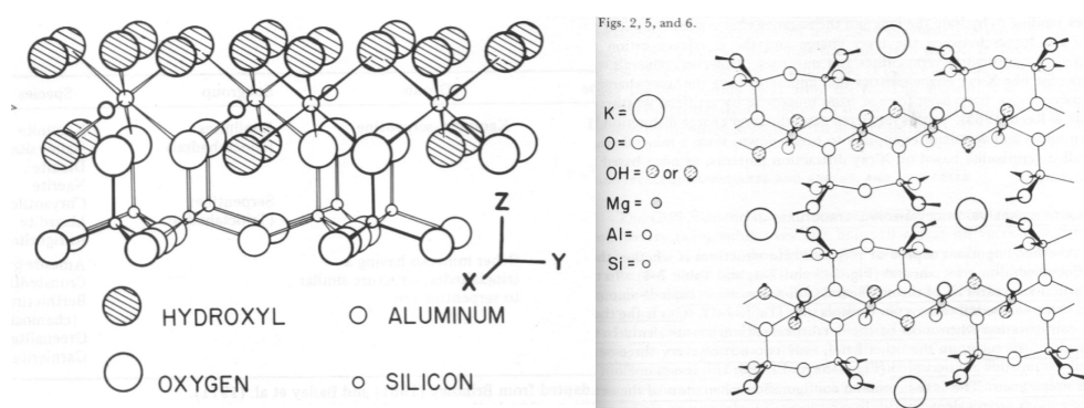
Figure 10. 1:1 Clay mineral (left) 2:1 clay mineral (right).
