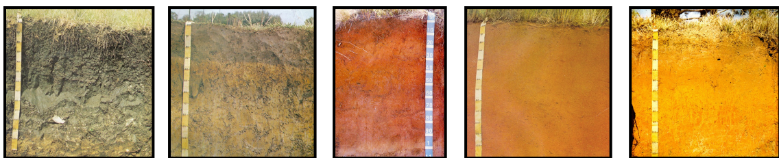
Figure 7. Soil types: Arcadia, Katspruit, Bainsvlei, Hutton and Avalon soils ( left to right ).
