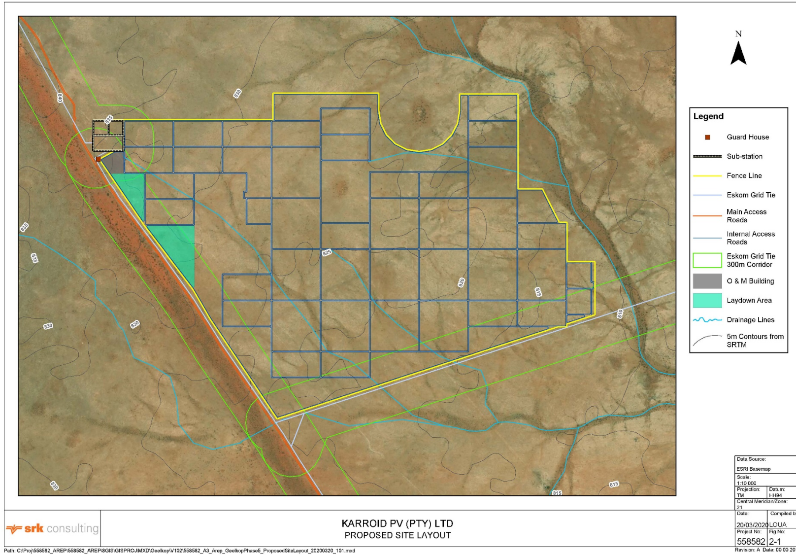
Figure 2-1: Karroid Conceptual Site Layout
