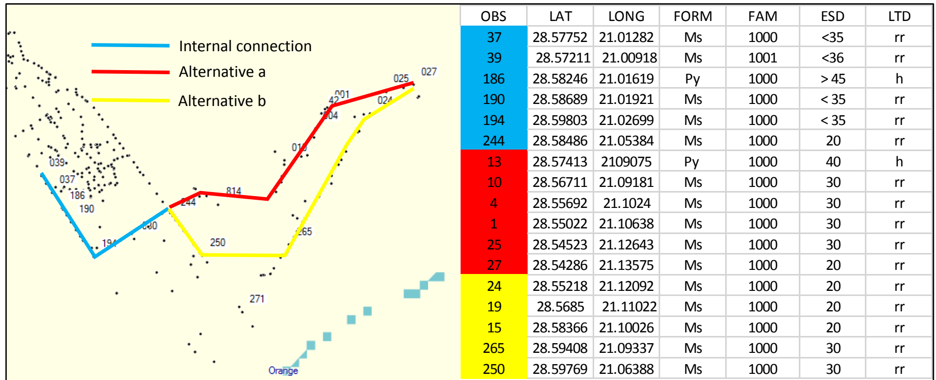
Figure 11: Grid connection alternatives proposed.
