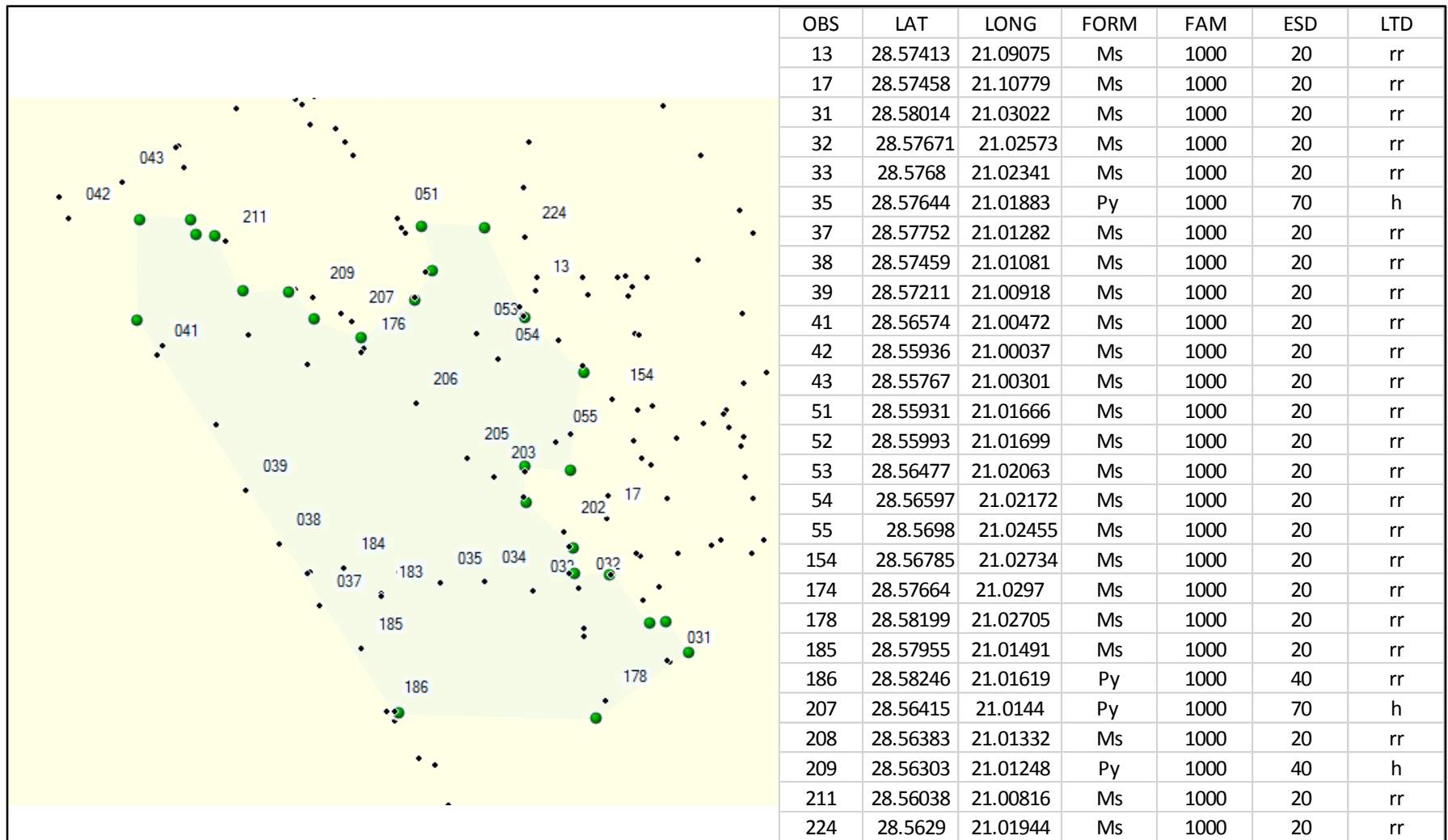
Figure 7: Soil survey
