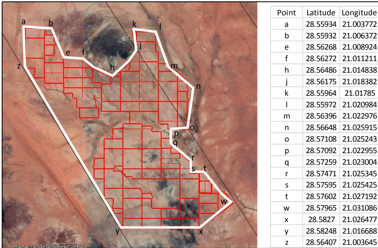
Figure 2: Proposed Layout of Site
