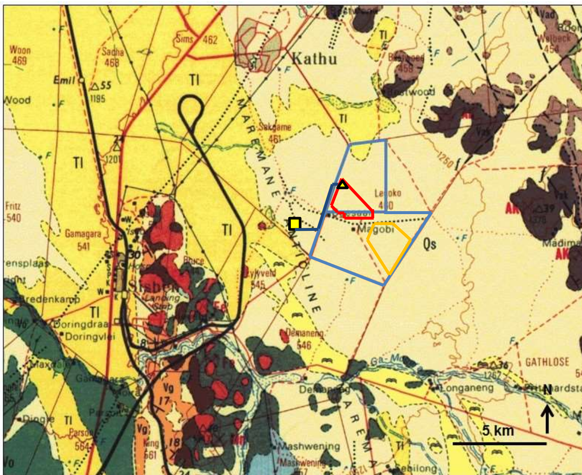
Fig. 3. Extract from 1: 250 000 geological map 2722 Kuruman (Council for Geoscience, Pretoria) showing the location of the study area for the proposed Mogara Solar PV Energy Facility on Portions 1 & 2 of Farm 460 Legoko (blue polygons) to the southeast of Kathu and east of the Sishen Mine. Note that the road and railway networks shown here are out of date (e.g. current route of N14 not shown). Red polygon = preferred PV solar site (red). Orange polygon = alternative PV solar site. Yellow square = Sekgame Switching Station. Dark blue line = 132 kV overhead transmission line from on-site substation (yellow triangle).
