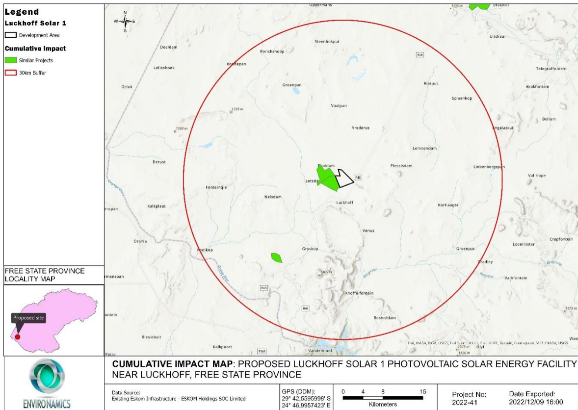
Figure 7: Luckhoff Solar 1 Solar Energy Facility: Geographic area of evaluation with utility-scale renewable energy generation sites and power lines.
