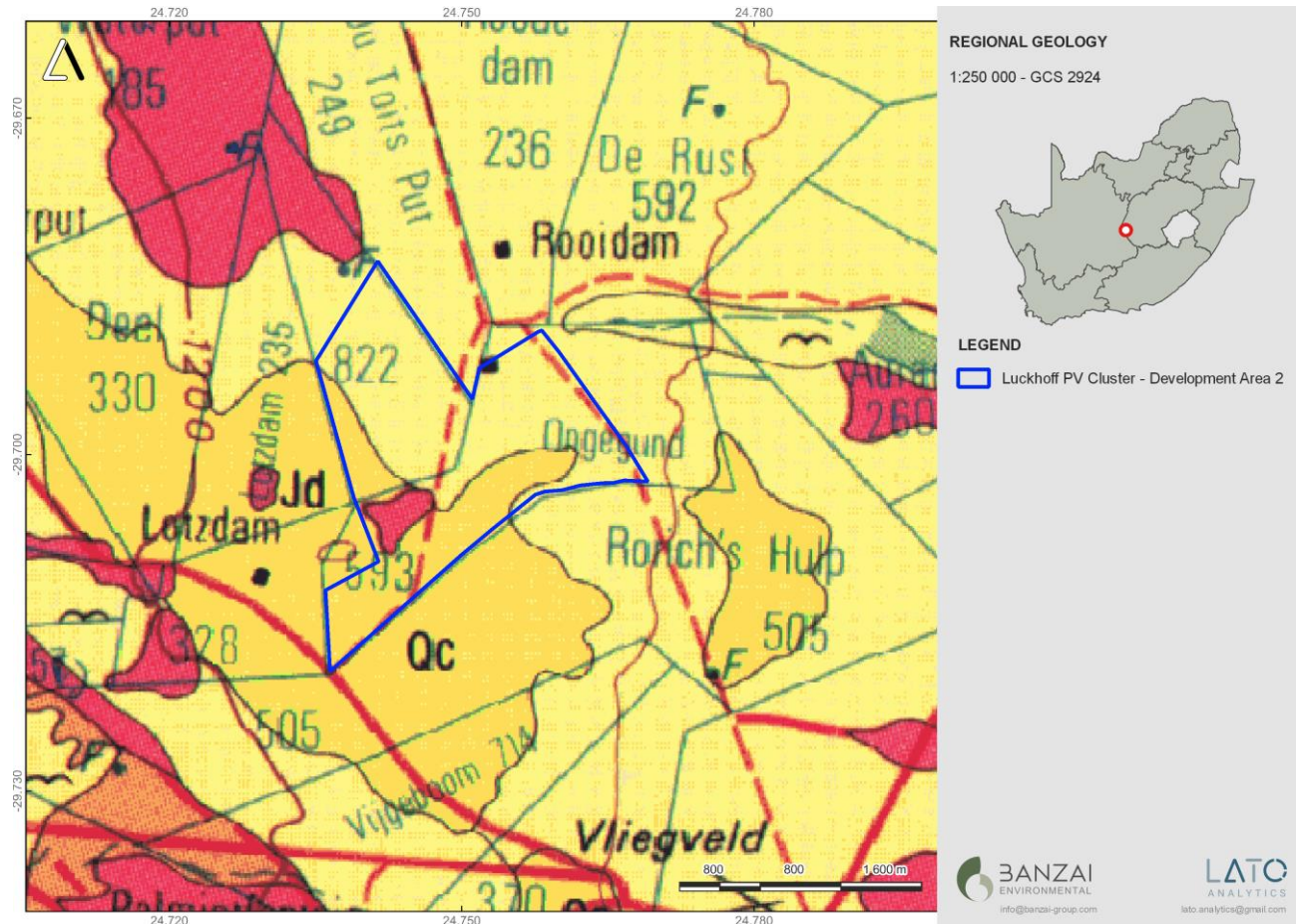
Figure 4: Extract of the 1:250 000 Koffiefontein 2924 Geological map (1992) (Council of Geoscience, Pretoria) indicating the geology of the Luckhoff Solar 2 Solar Energy Facility in the Free State Province. The development is underlain by Cenozoic aeolian sand (Qs), calcrete (Qc, yellow) as well as a small portion of Jurassic dolerite (Jd,
