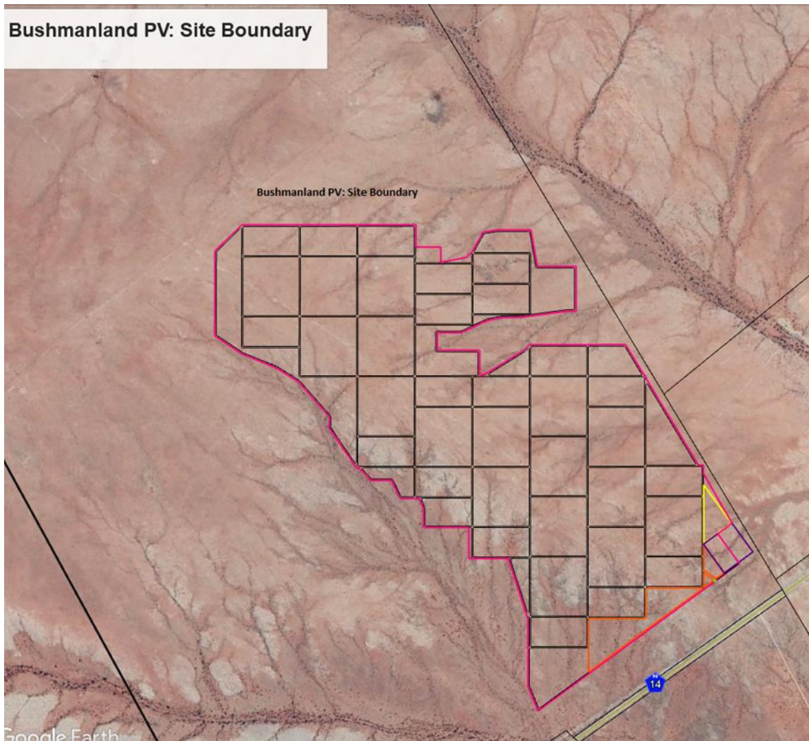
Figure 4: Bushmanland PV Site Development Boundary
