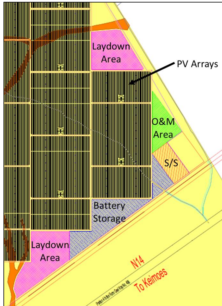
Figure 8: Proposed layout indicating battery storage area.
