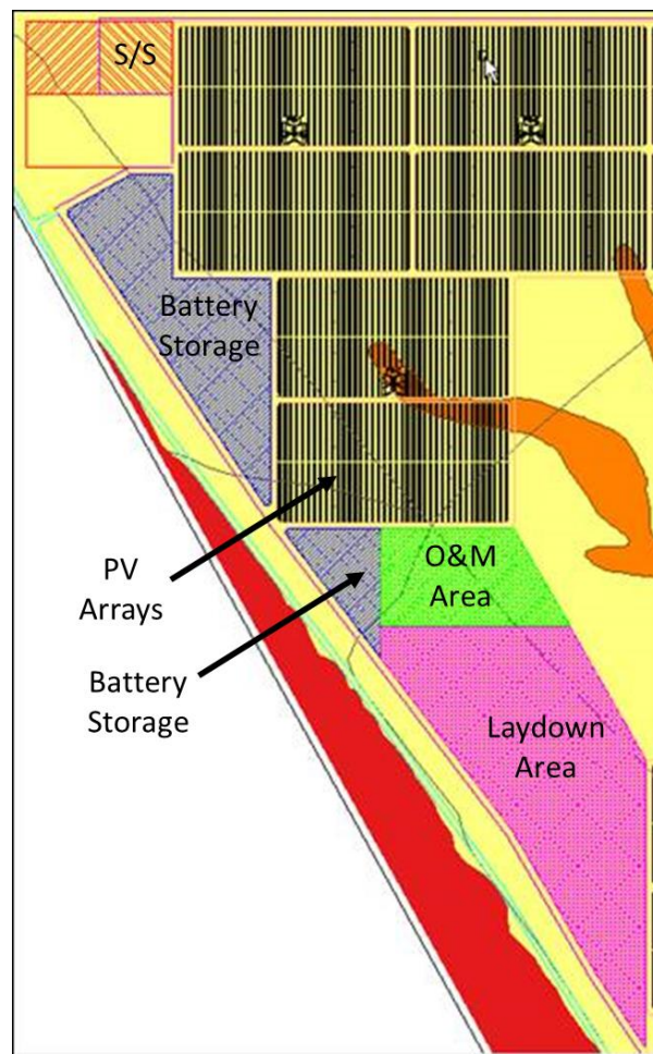
Figure 8: Proposed layout indicating battery storage area.
