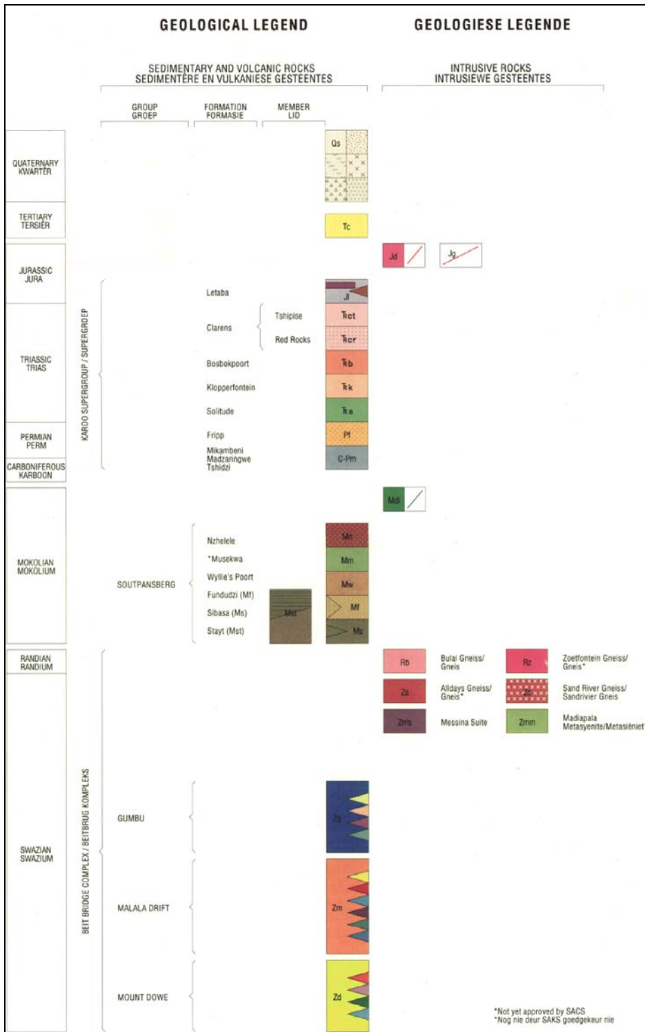
Figure 3: Geological map and legend.
