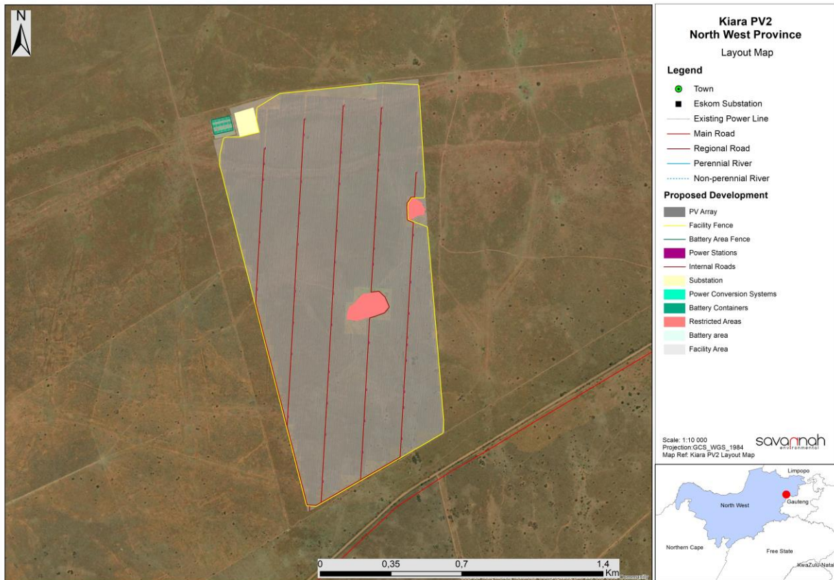
Figure 11 Layout of the Kiara PV 2 facility's infrastructure.
