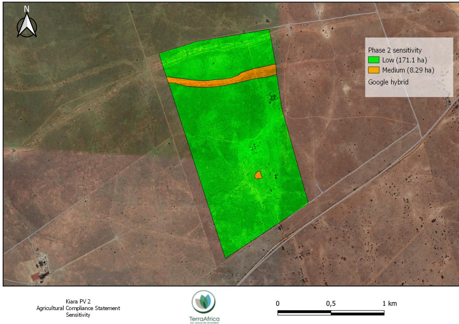
Figure 10: Agricultural sensitivity rating of the proposed Kiara PV 2 facility development area
