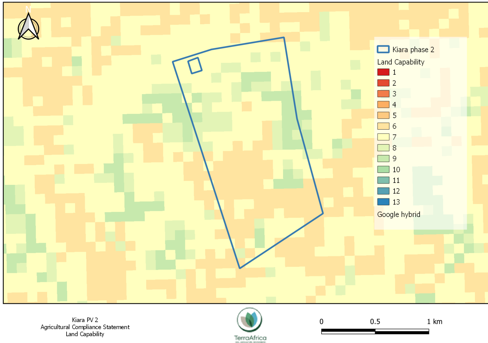
Figure 5 Land capability classification of the Kiara PV 2 development area (data source: DALRRD, 2016).
