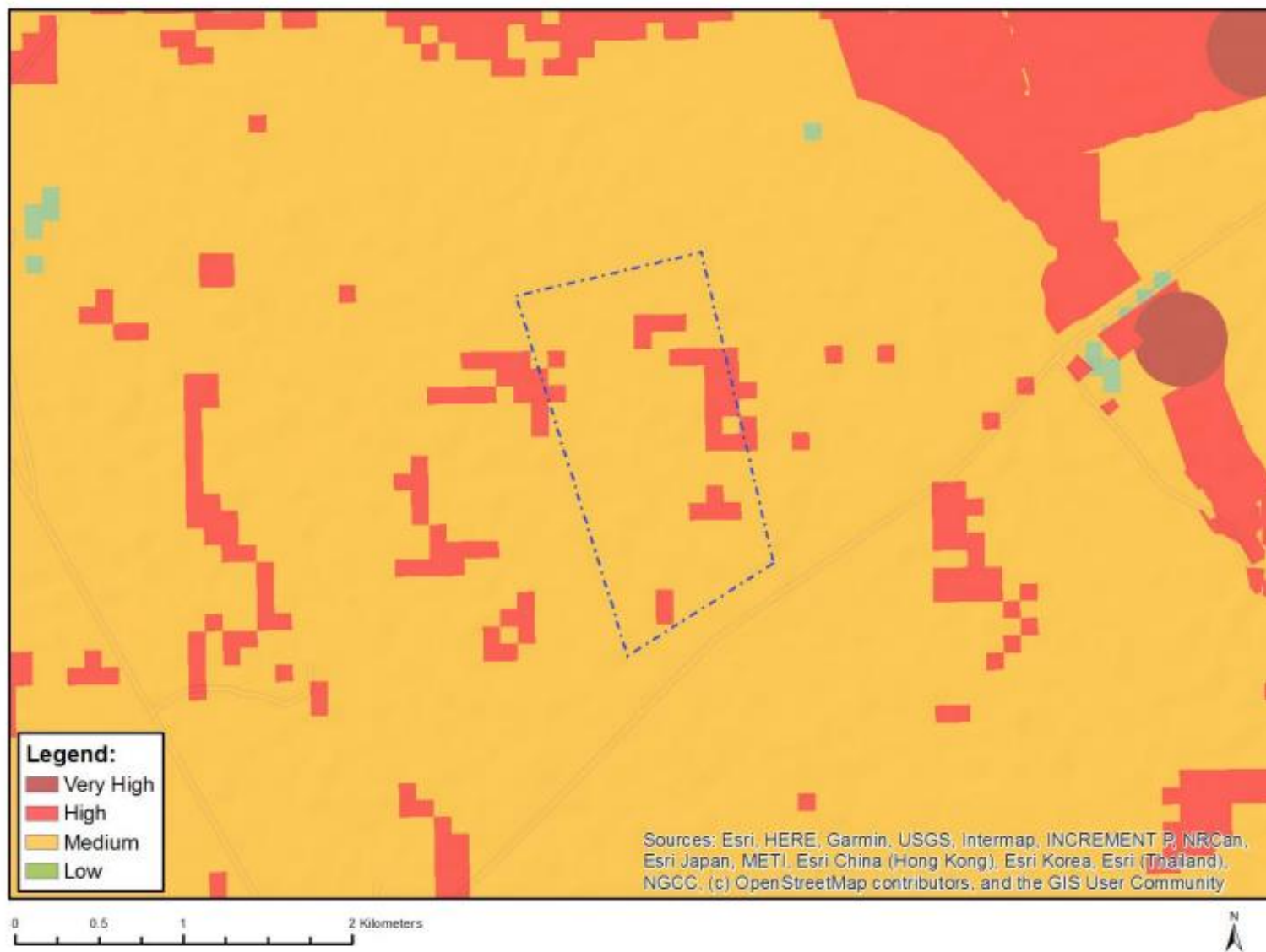
Figure 1 Agricultural Combined Sensitivity of the Kiara PV 2 development area (generated by Savannah Environmental, 2022)
