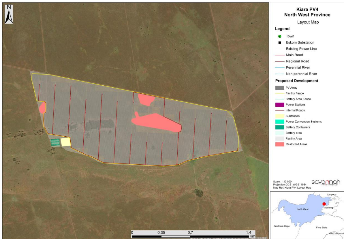
Figure 11 Layout of the Kiara PV 4 facility's infrastructure.
