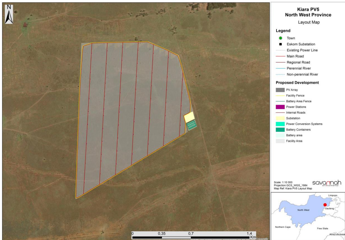
Figure 11 Layout of the Kiara PV 5 facility's infrastructure.
