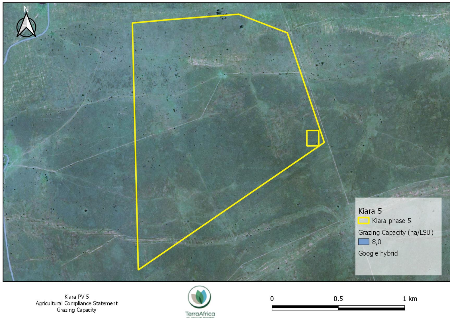
Figure 9: Grazing capacity of the Kiara PV 5 development area (data source: DALRRD, 2018).
