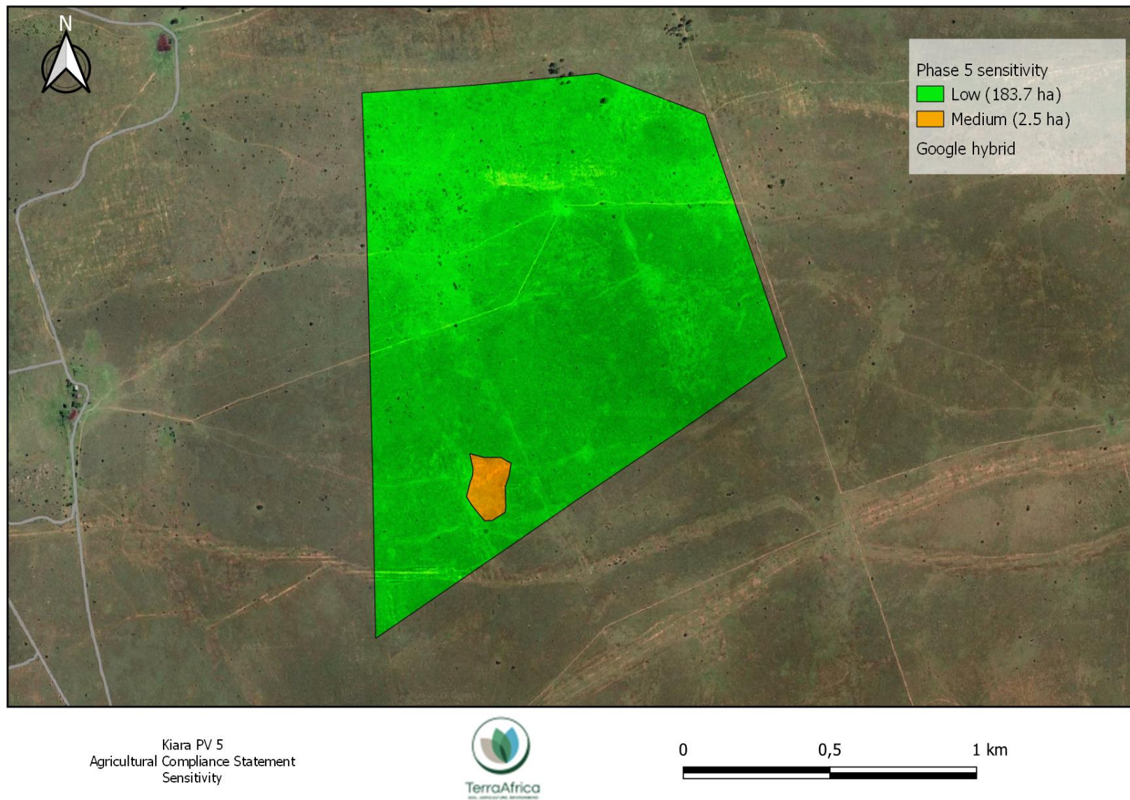
Figure 10: Agricultural sensitivity rating of the proposed Kiara PV 5 facility development area
