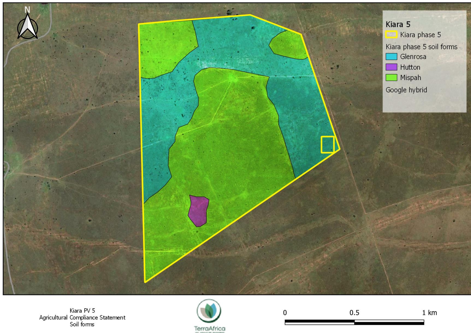
Figure 3: Soil classification map of the Kiara PV 5 development area
