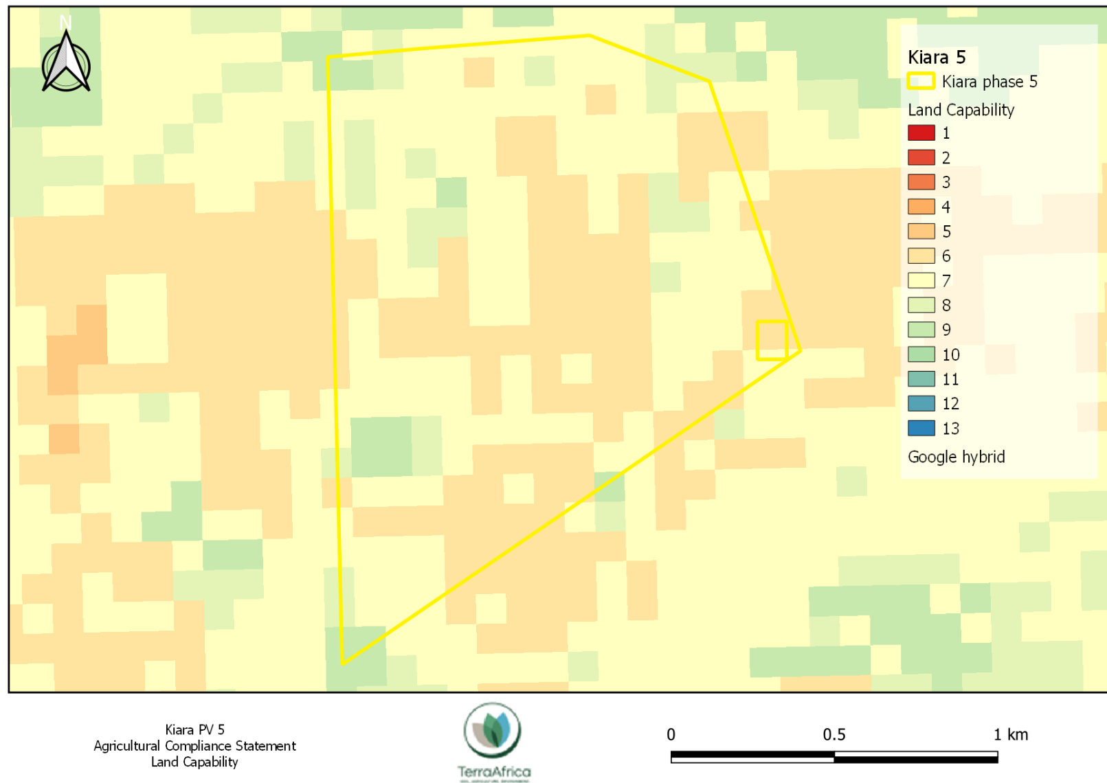
Figure 5 Land capability classification of the Kiara PV 5 development area (data source: DALRRD, 2016).
