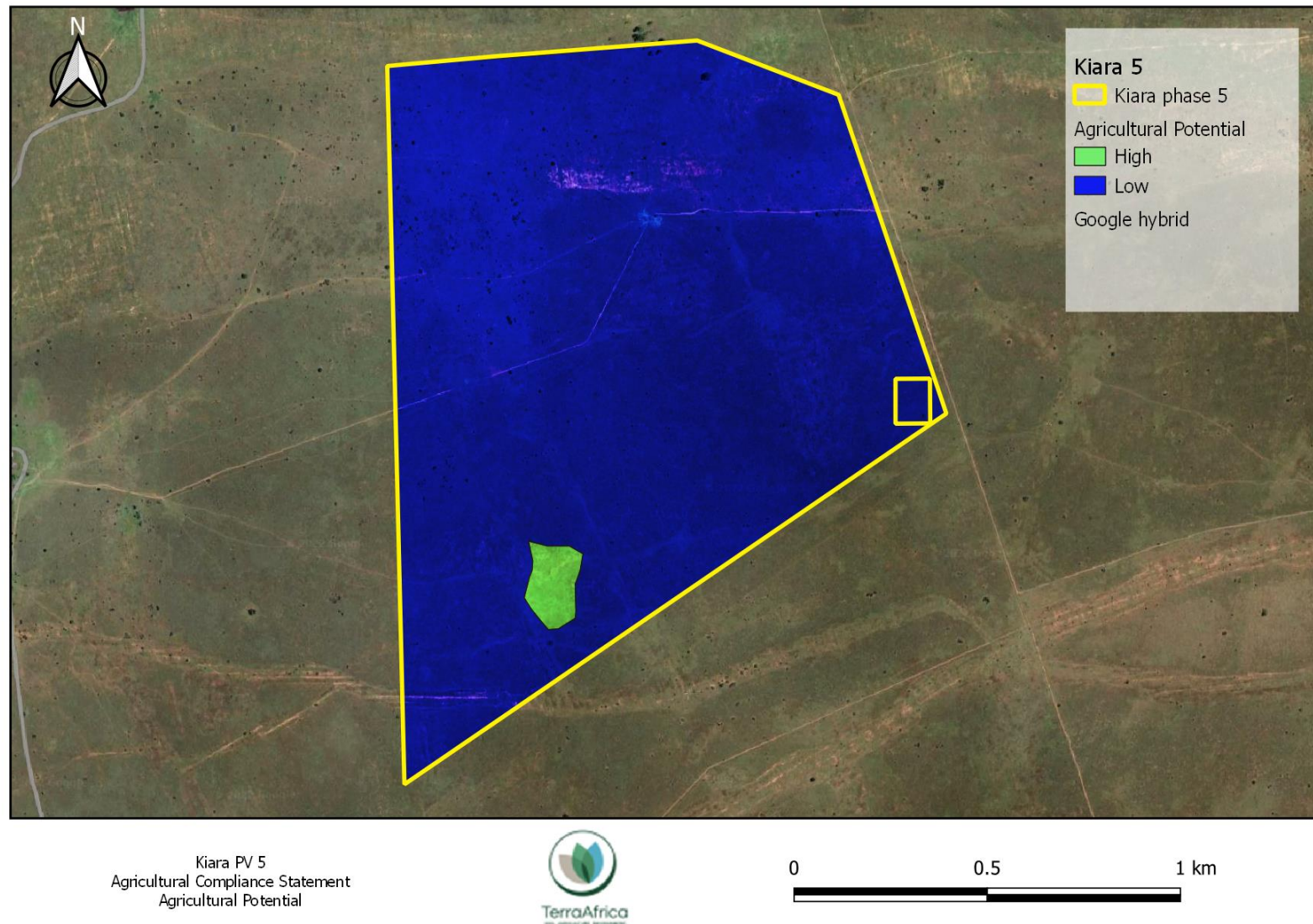
Figure 7: Agricultural potential of the Kiara PV 5 development area
