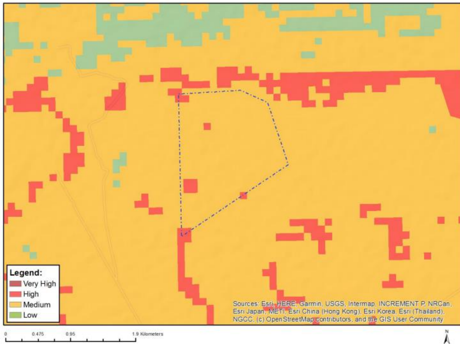
Figure 1 Agricultural Combined Sensitivity of the Kiara PV 5 development area (generated by Savannah Environmental, 2022)
