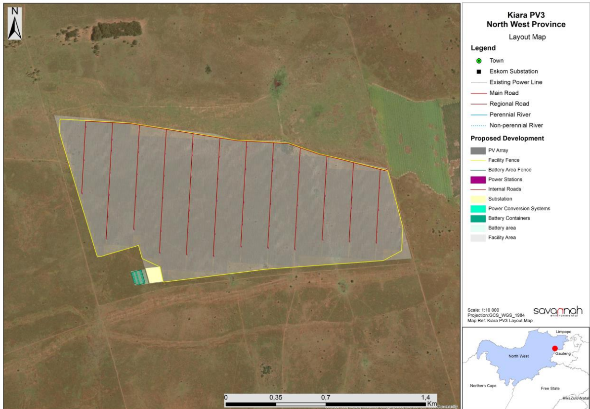
Figure 11 Layout of the Kiara PV 3 facility's infrastructure.
