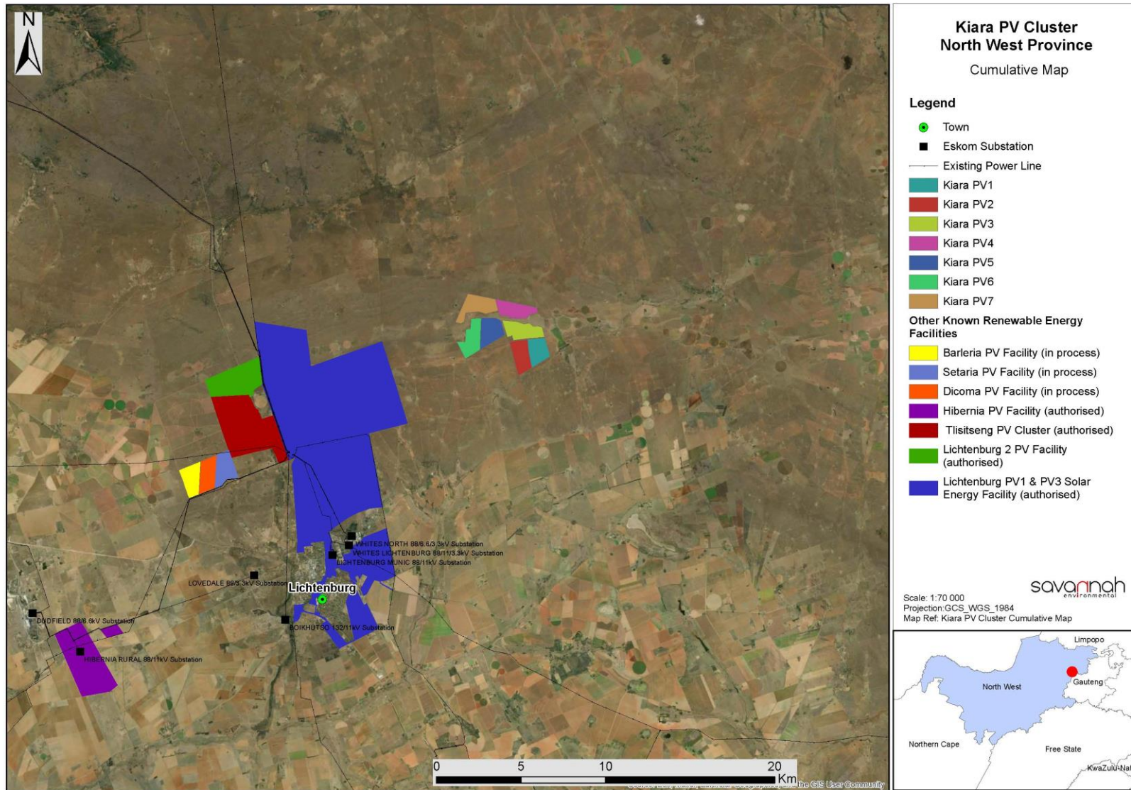
Figure 11 Projects around the proposed Kiara PV 3 Facility that may result in cumulative impacts
