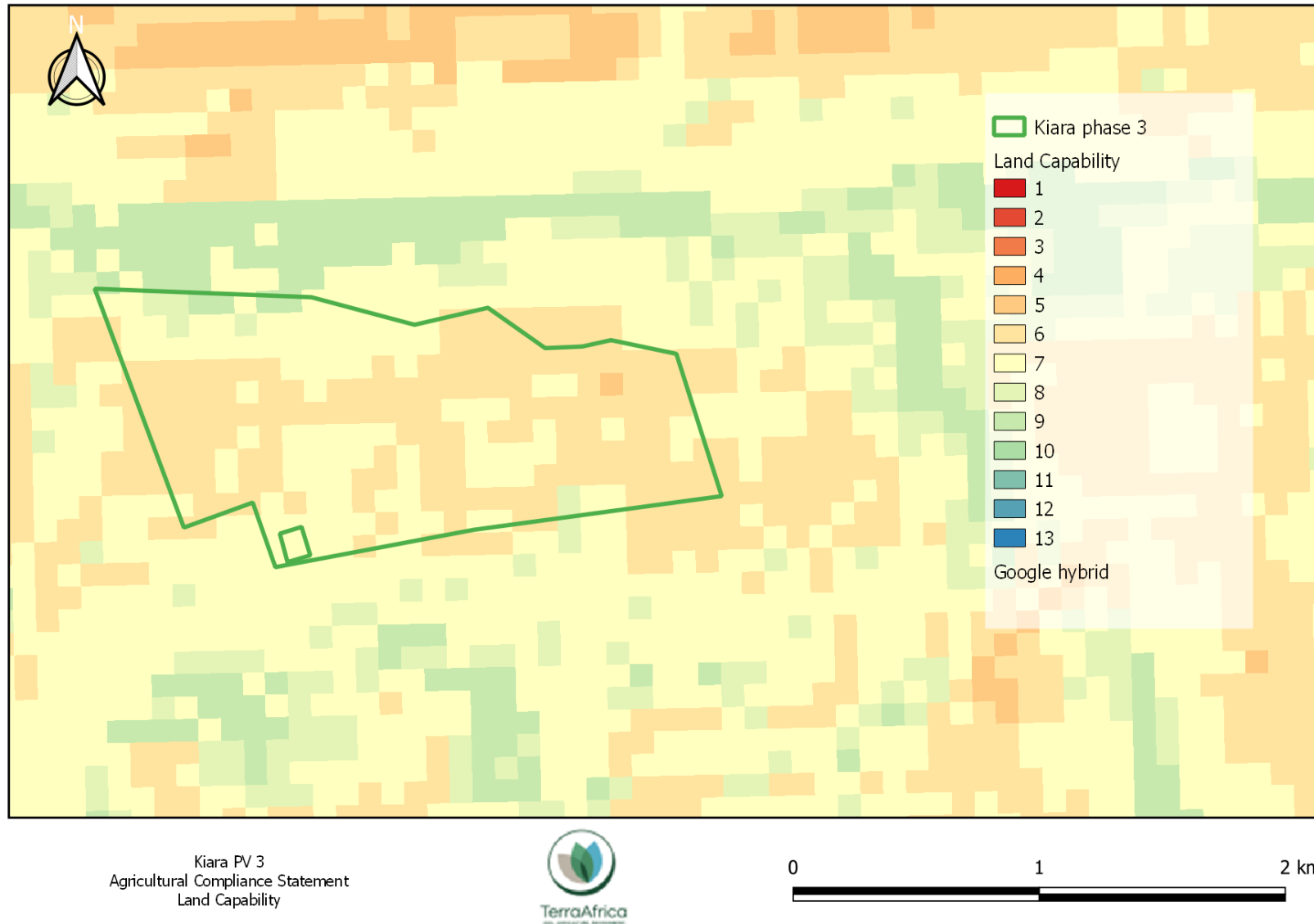
Figure 5 Land capability classification of the Kiara PV 3 development area (data source: DALRRD, 2016).
