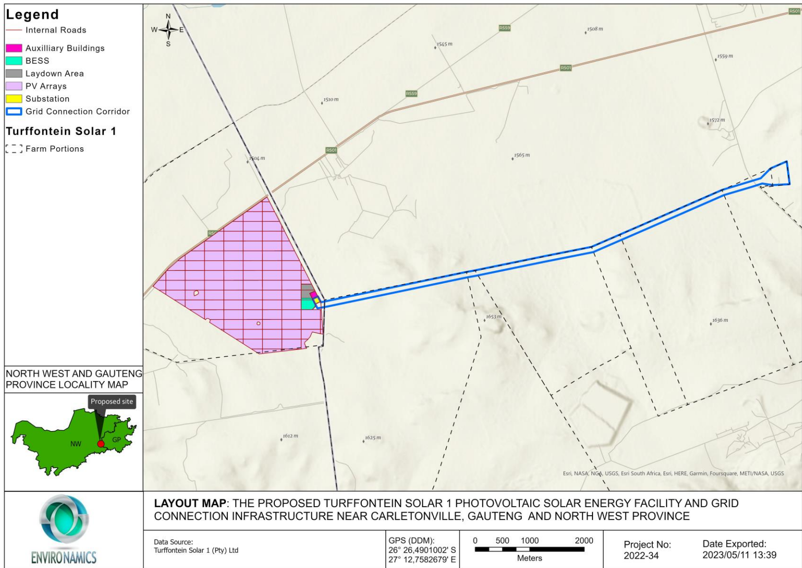
Figure 1: Layout plan indicating the proposed development footprint
