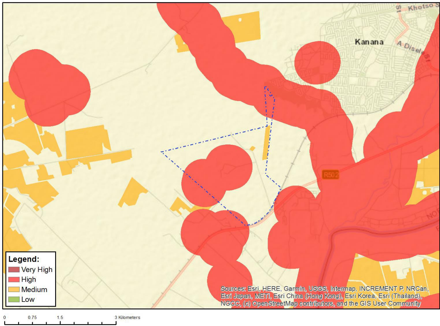
Figure 6: Map of the relative avian theme sensitivity
