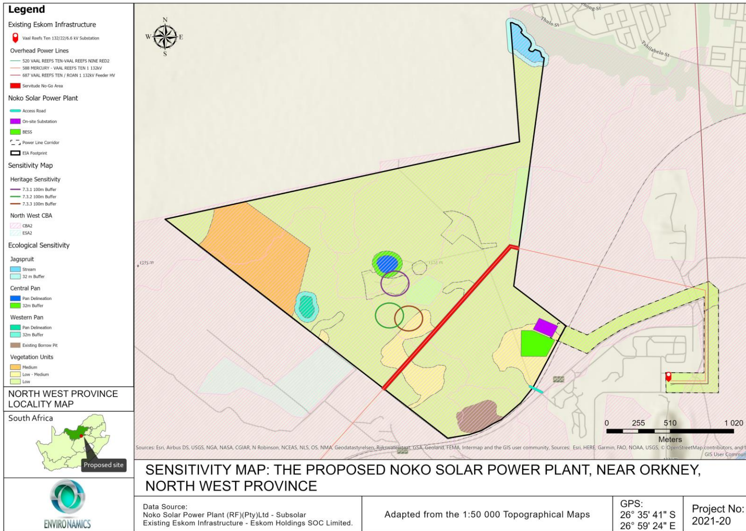
Figure 1: Environmental sensitivity map of the Noko Solar Power Plant
