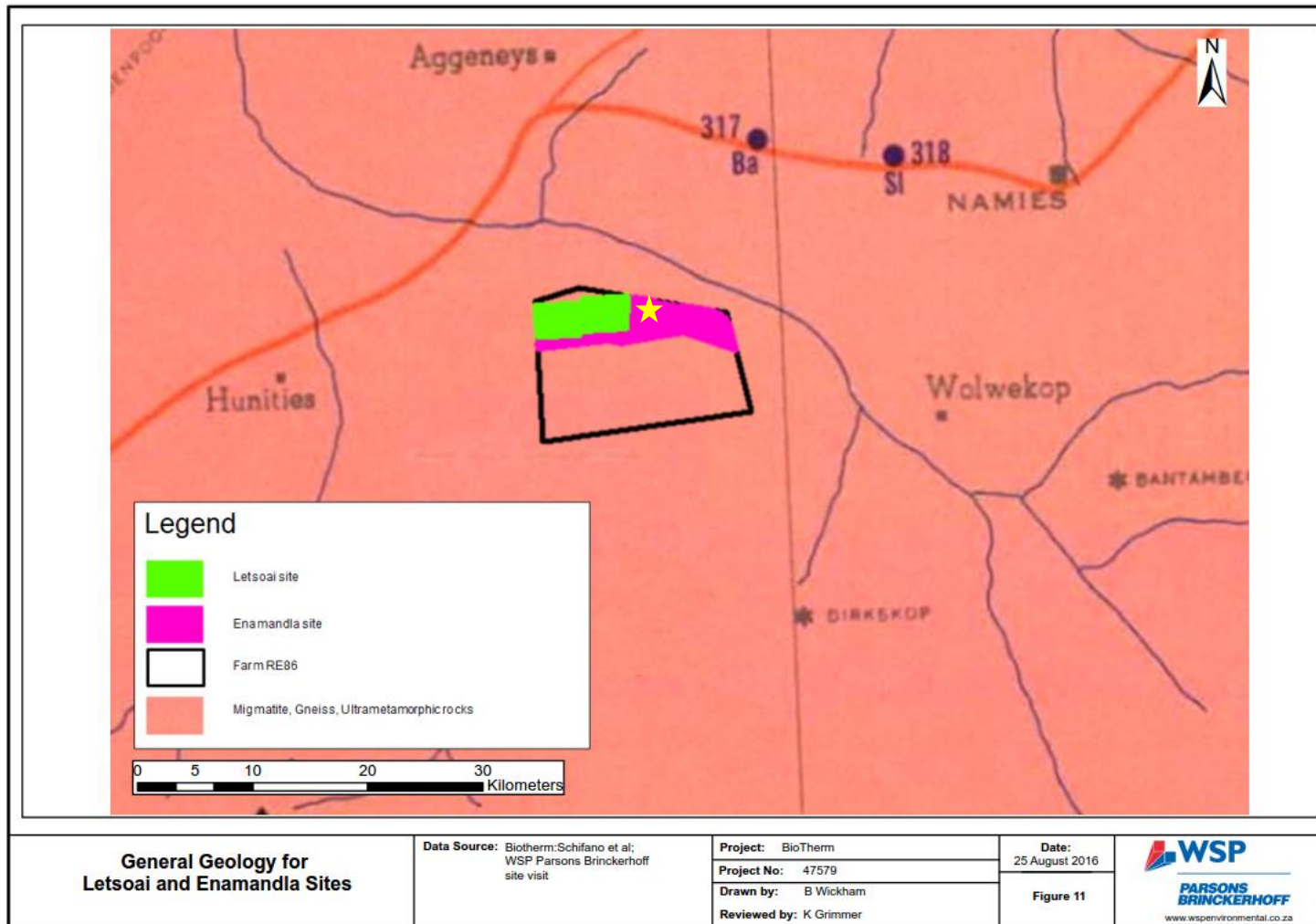
Figure 11 General Geology for Letsoai and Enamandla Sites (Yellow star denotes location of Enamandla PV Site 1)
