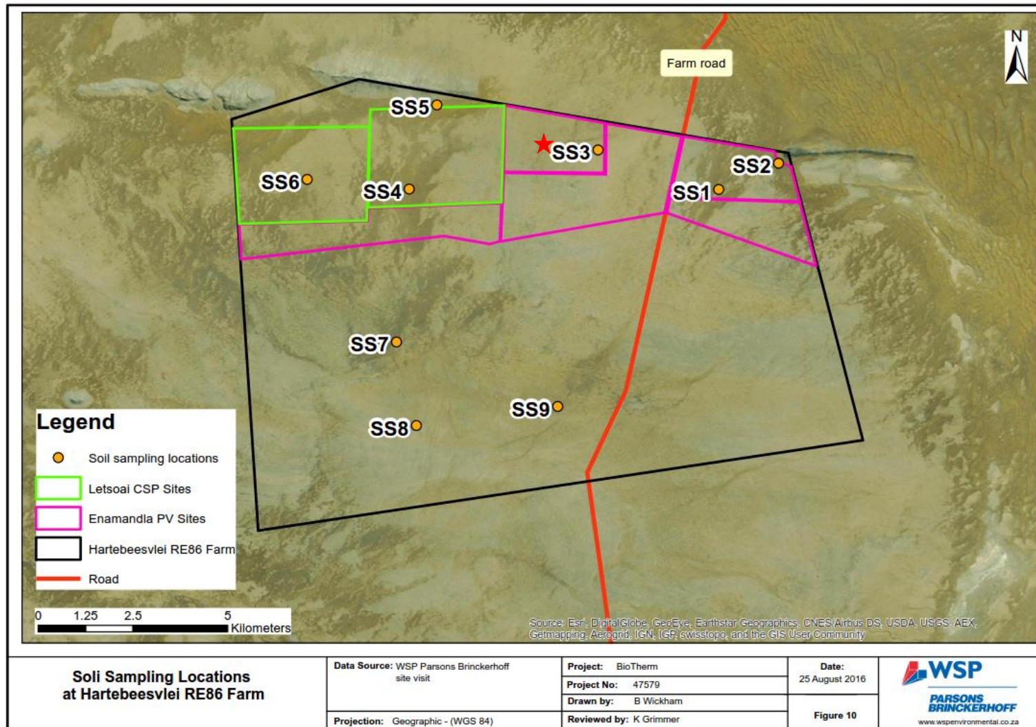
Figure 9 Soil Sampling Locations within Hartebeesvlei RE86 Farm (Red star denotes the location of Enamandla PV Site 1)
