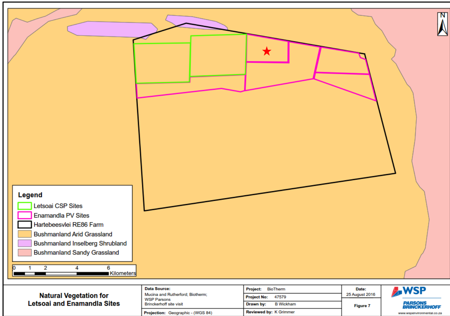
Figure 6 Natural Vegetation for Letsoai CSP and Enamandla PV Sites (Red star denotes location of Enamandla PV Site 1)
