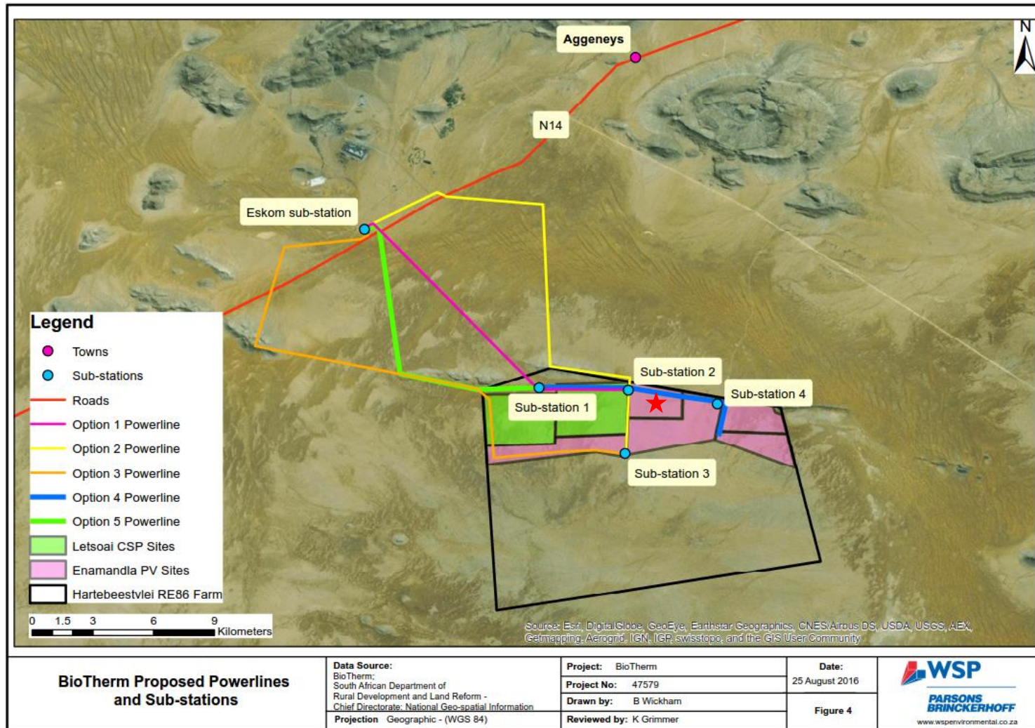
Figure 3 BioTherm Proposed Powerlines and Sub-Stations (Red star denotes location of Enamandla PV Site 1)
