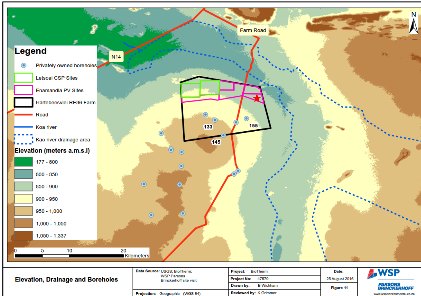
Figure 10 Elevation, Drainage and Boreholes (Red star denotes location of Enamandla PV Site 5)
