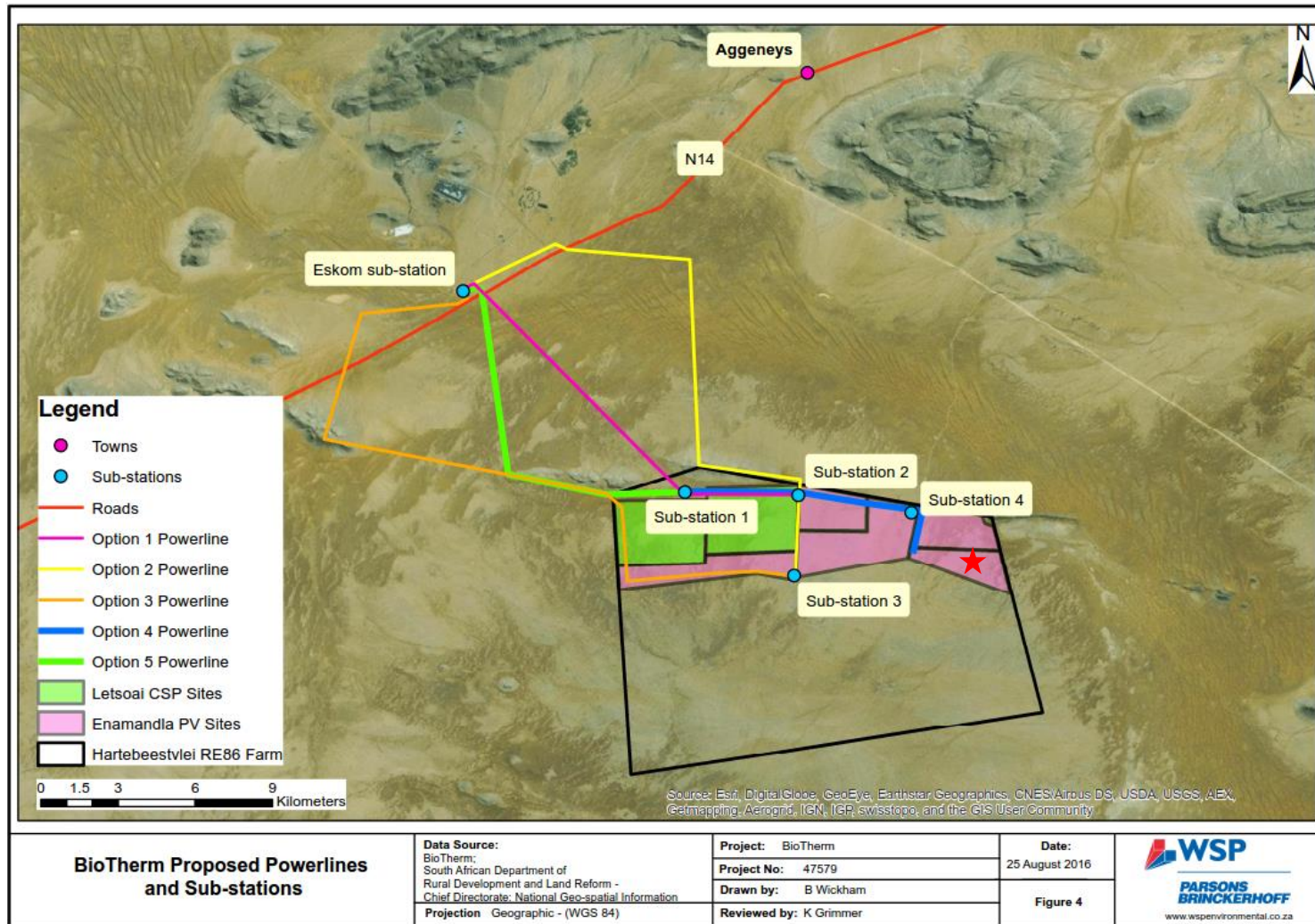
Figure 3 BioTherm Proposed Powerlines and Sub-Stations (Red star denotes location of Enamandla PV Site 5)
