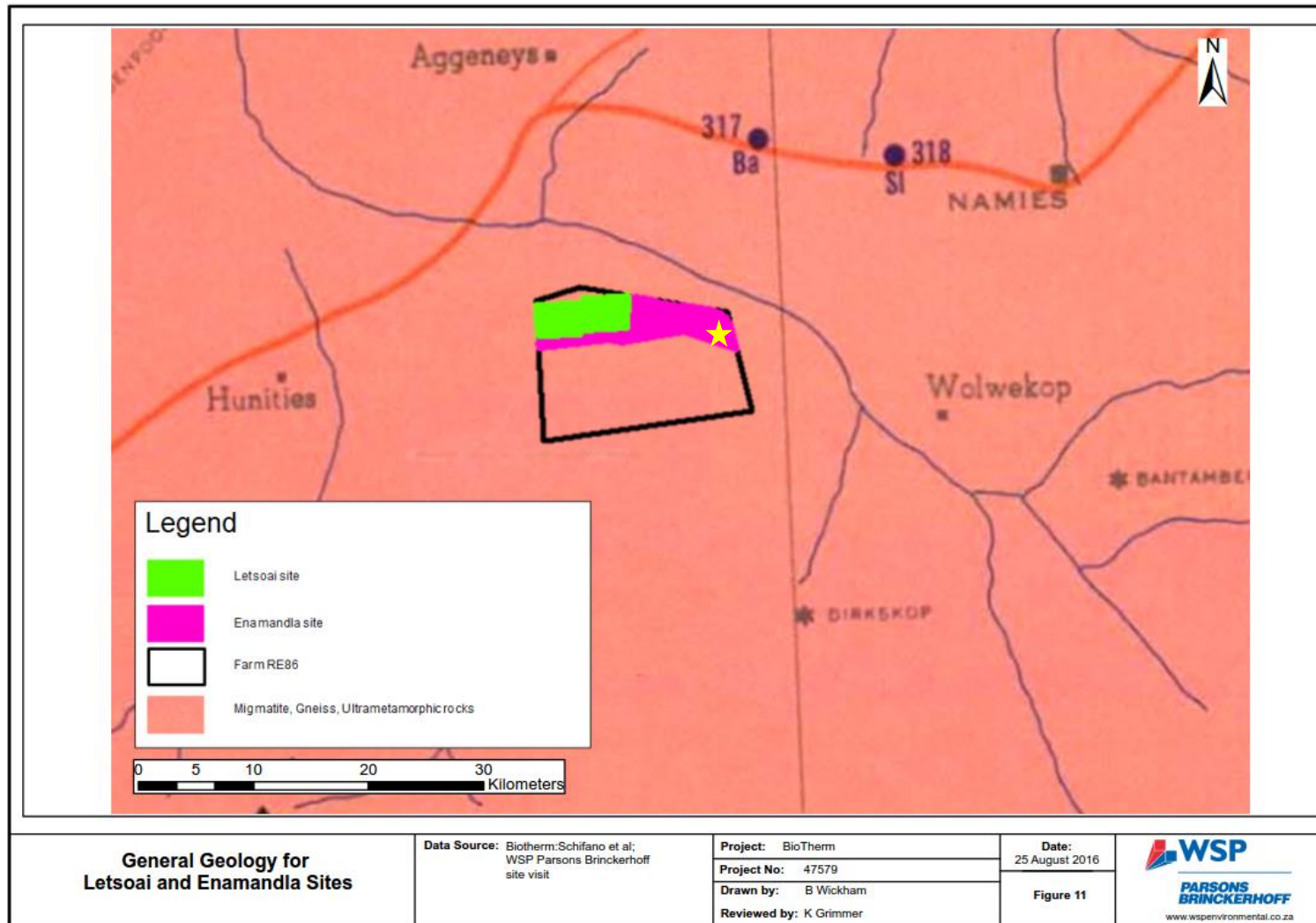
Figure 11 General Geology for Letsoai and Enamandla Sites (Yellow star denotes location of Enamandla PV Site 5)
