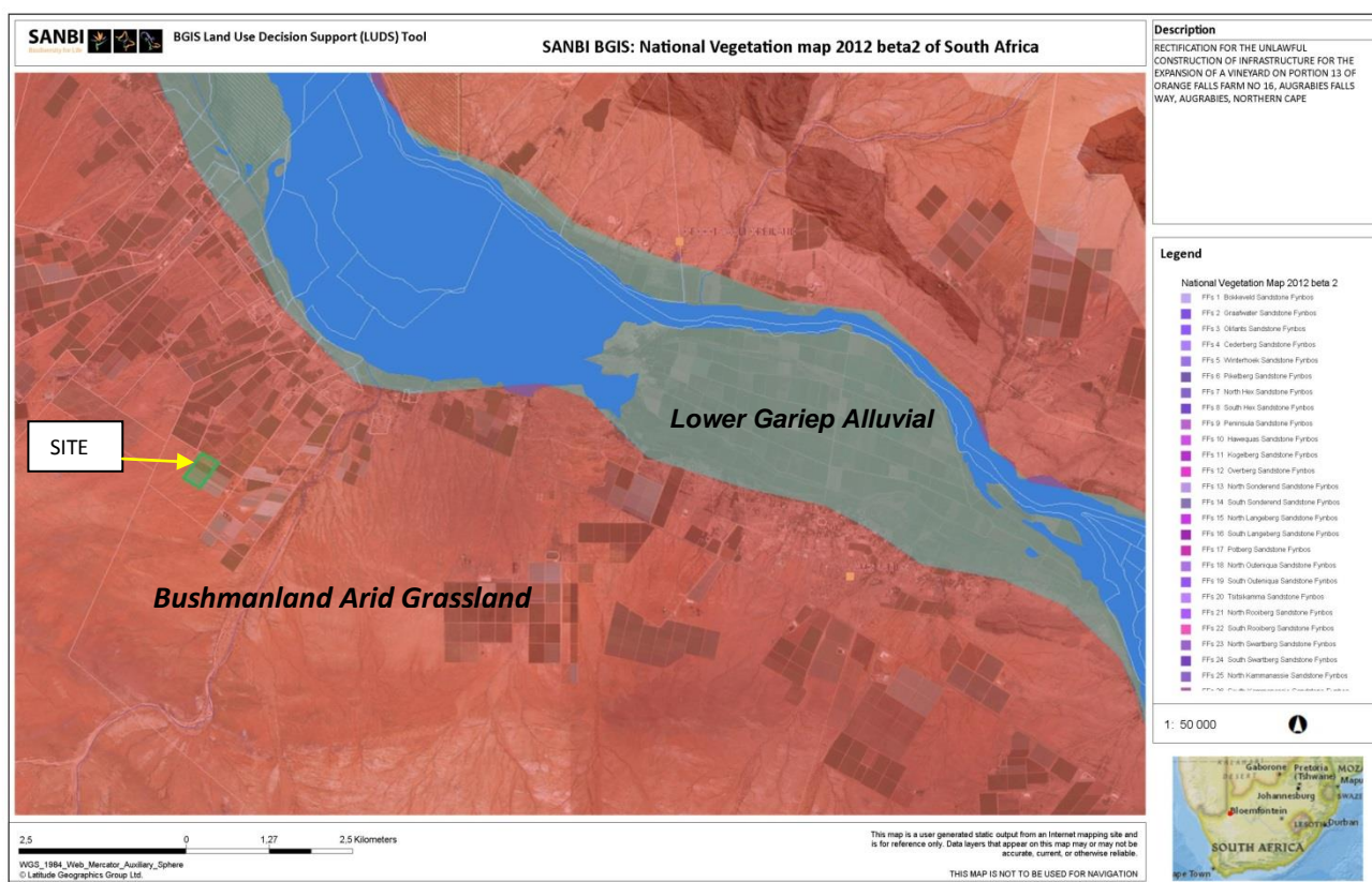
Figure 4: SANBI BGIS - The National vegetation map of SA, indicating the vegetation on the site.
