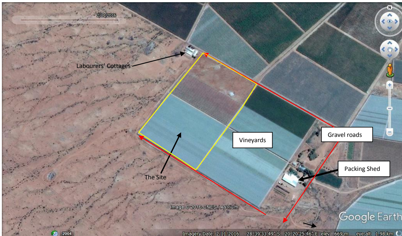
Figure 3: Aerial image of the site (yellow rectangle) and its surroundings. Access roads indicated by the red arrows.
