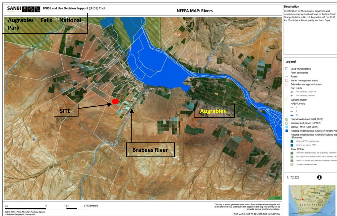
Figure 6: NFEPA (National Freshwater Ecosystem Priority Areas) Map of the proposed site (red dot) and its surroundings.
