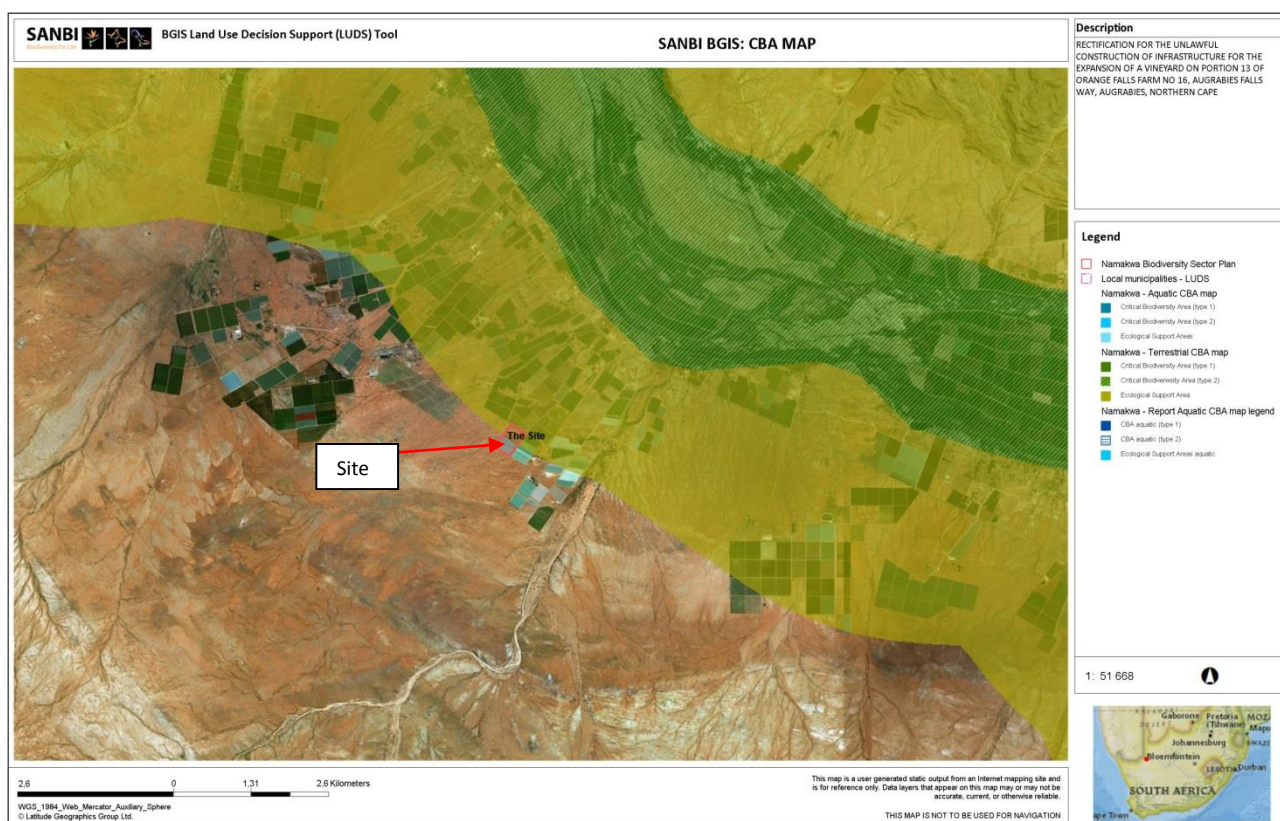
Figure 5: Threatened ecosystem map of the proposed site.
