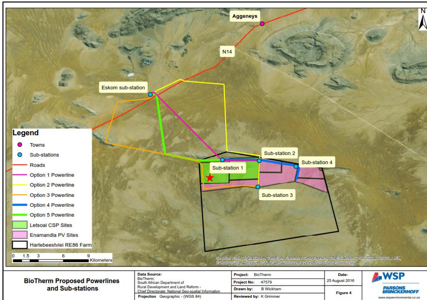
Figure 4 BioTherm Proposed Powerlines and Sub-Stations (Red star denotes location of Letsoai CSP Site 1)
