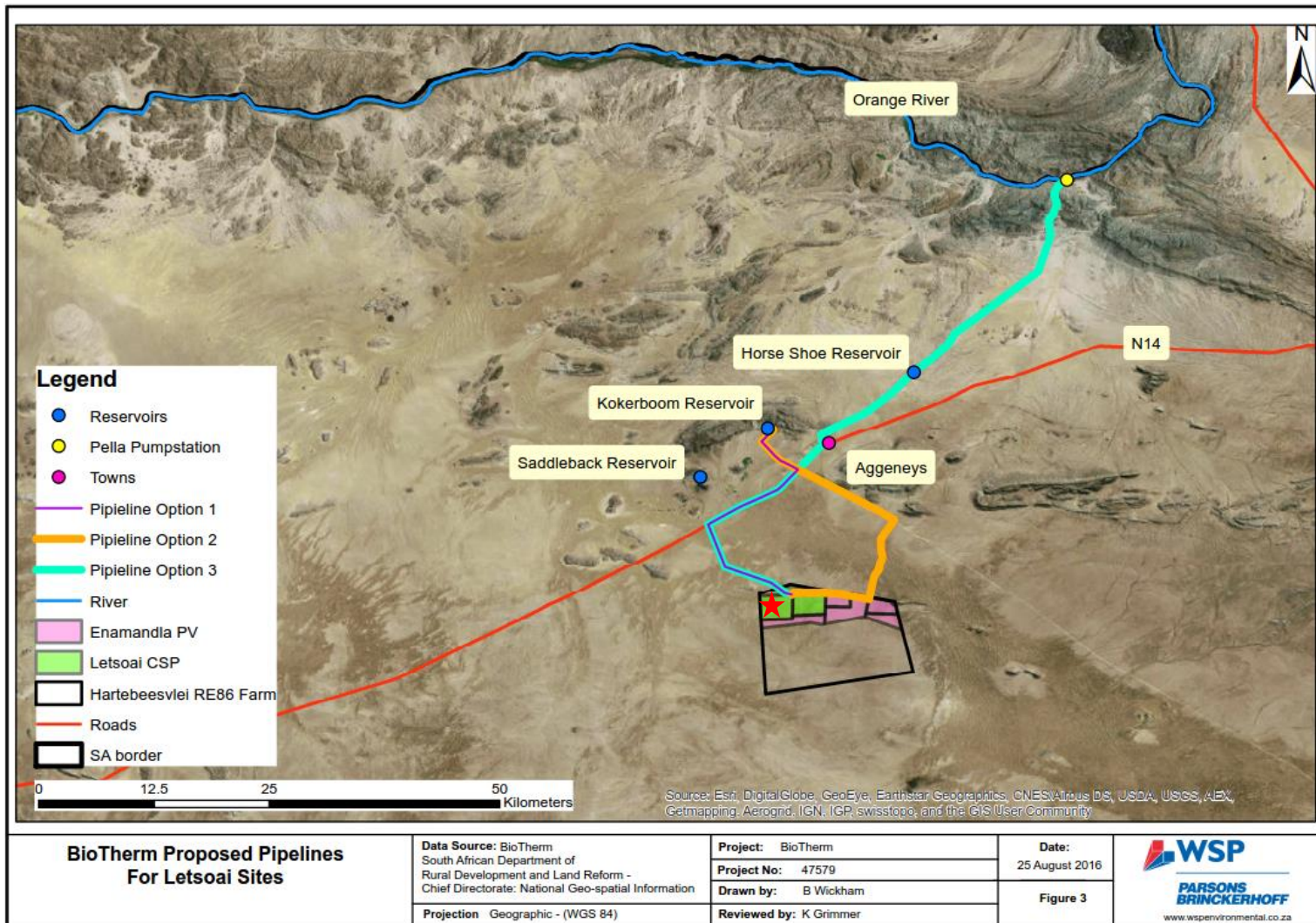
Figure 3 BioTherm Proposed Pipelines (Red star denotes location of Letsoai CSP Site 1)
