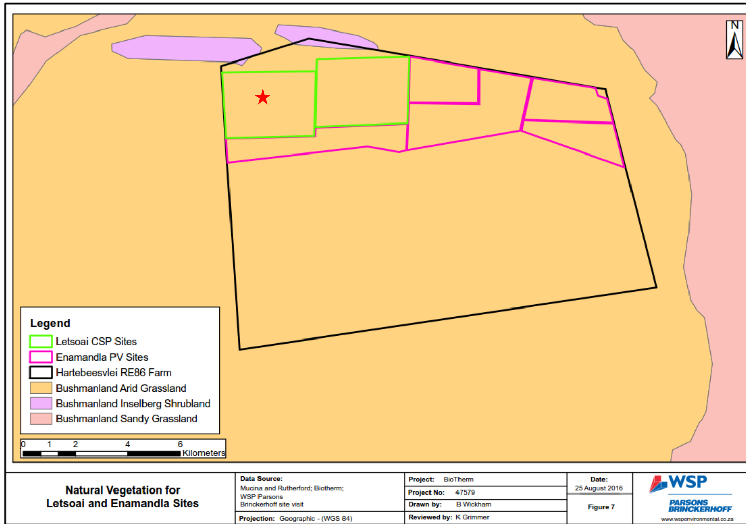
Figure 7 Natural Vegetation for Letsoai CSP and Enamandla PV Sites (Red star denotes location of Letsoai CSP site 1)
