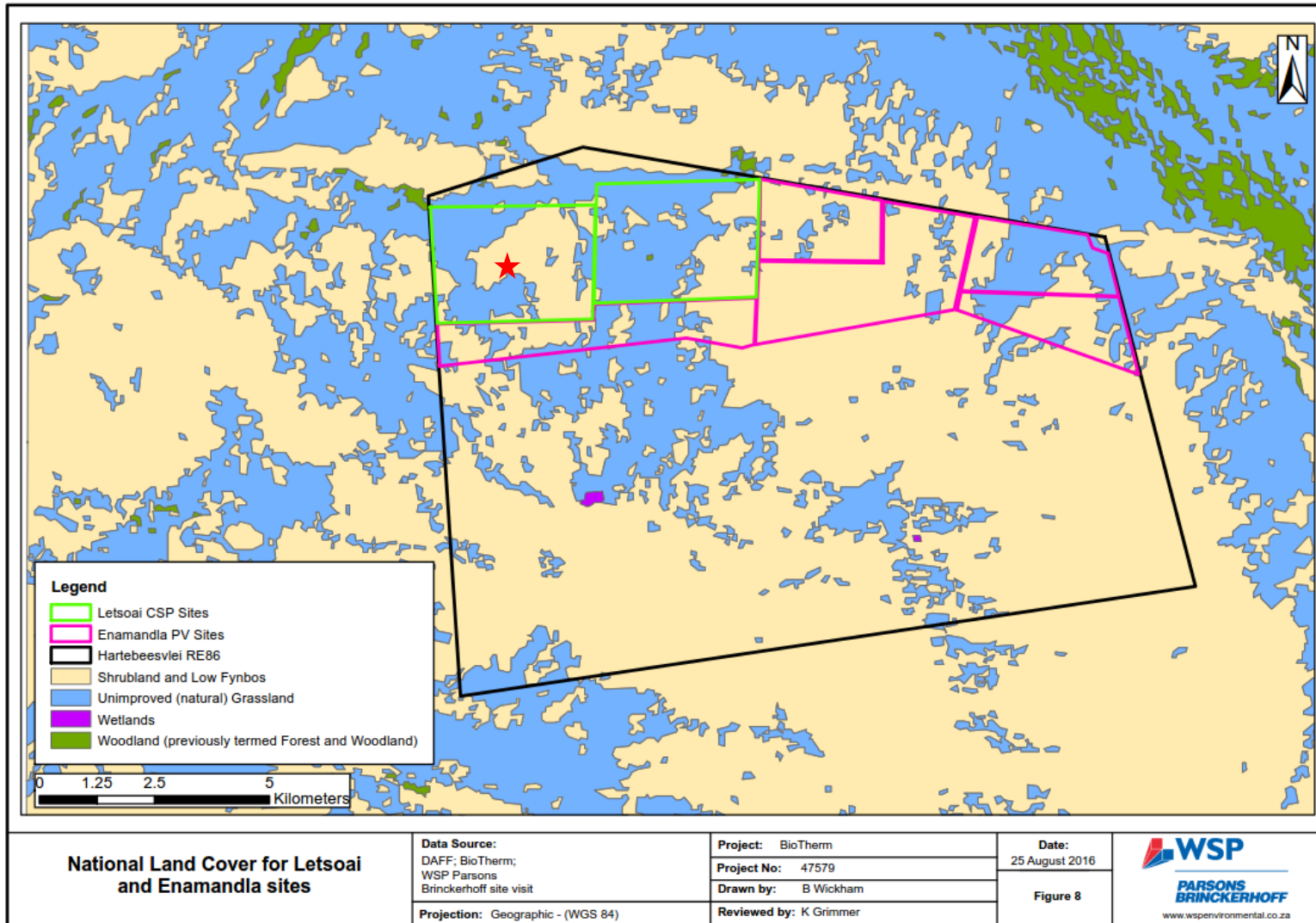
Figure 8 National Land Cover for Letsoai CSP and Enamandla PV Sites (Red star denotes location of Letsoai CSP site 1)
