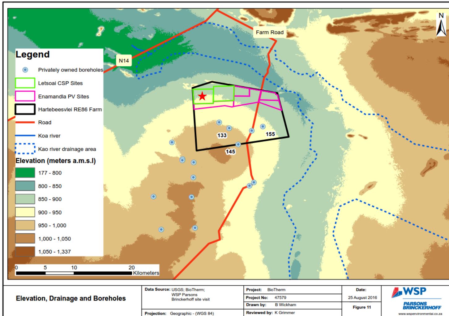
Figure 11 Elevation, Drainage and Boreholes (Red star denotes location of Letsoai CSP site 1)
