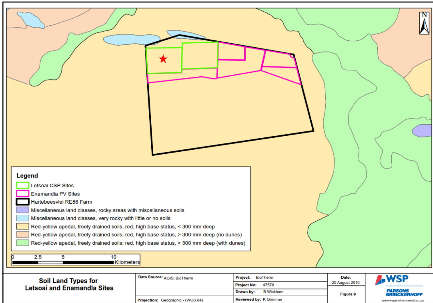
Figure 9 Soil land Types for Letsoai CSP and Enamandla PV Sites (Red star denotes location of Letsoai CSP site 1)
