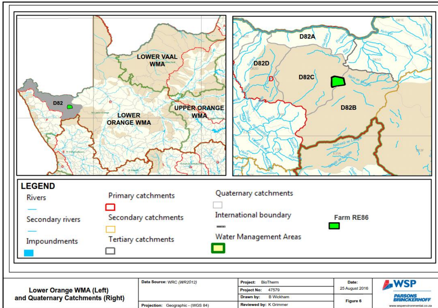
Figure 6 Lower Orange WMA (left) and Quaternary Catchments (right)
