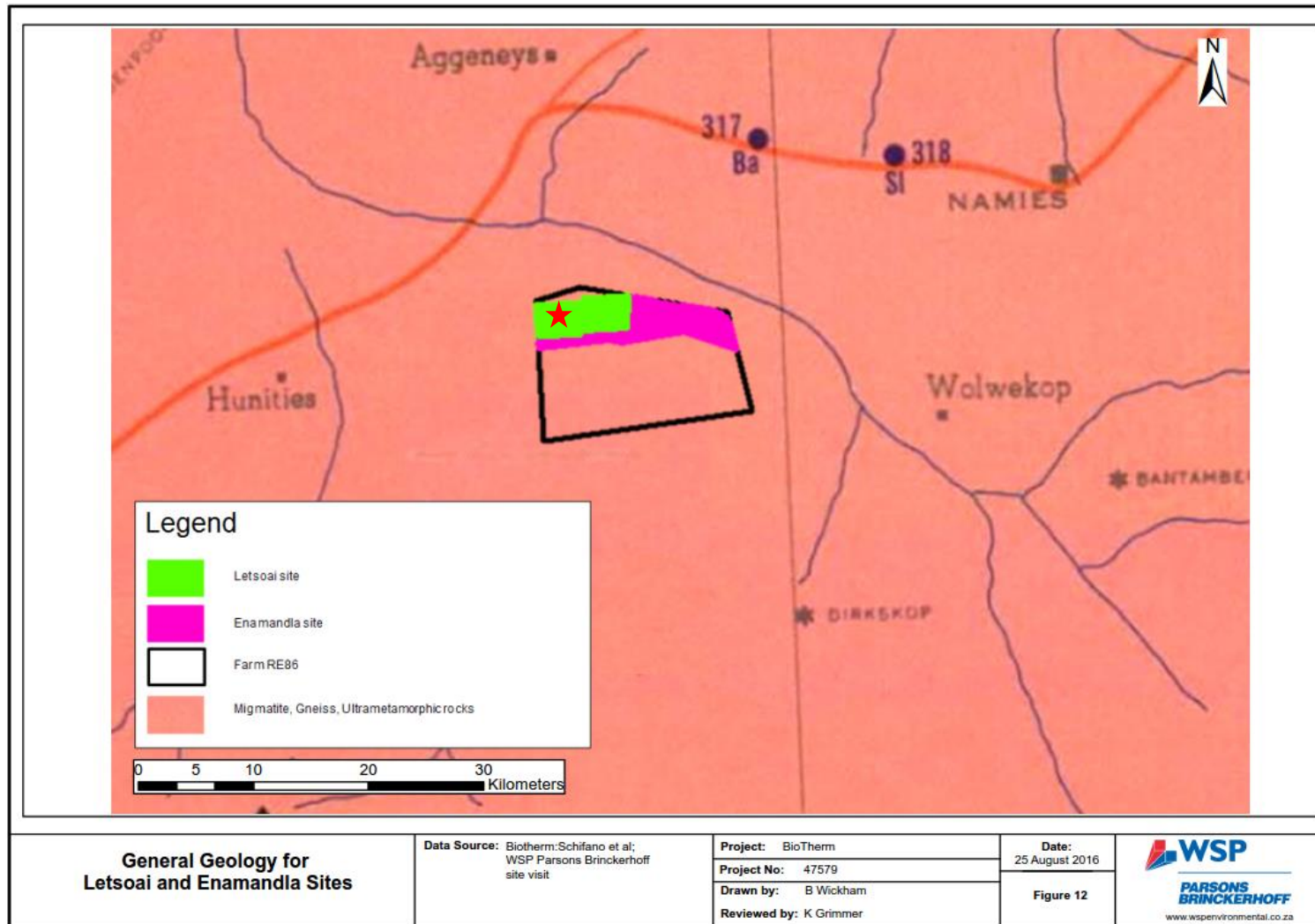
Figure 12 General Geology for Letsoai and Enamandla Sites (Red star denotes location of Letsoai CSP site 1)
