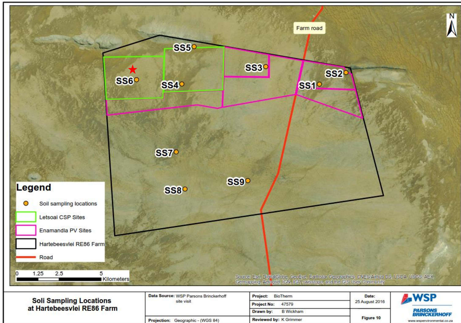
Figure 10 Soil Sampling Locations within Hartebeesvlei RE86 Farm (Red star denotes the location of Letsoai CSP site 1)
