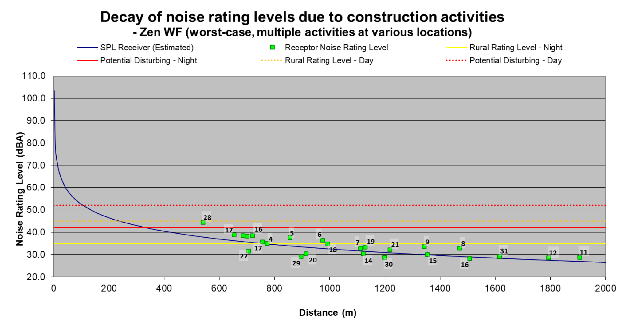
Figure 9-3: Projected conceptual construction noise levels for the proposed Zen WF
