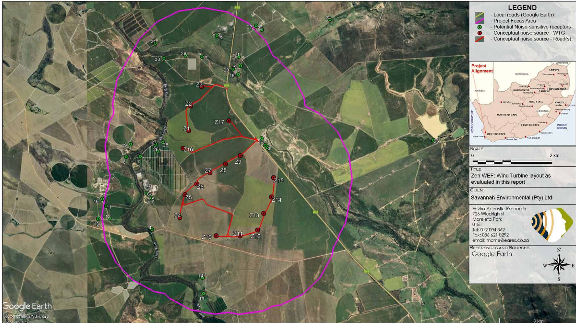
Figure 9-1: WTG locations and associated infrastructure for the proposed Zen WF
