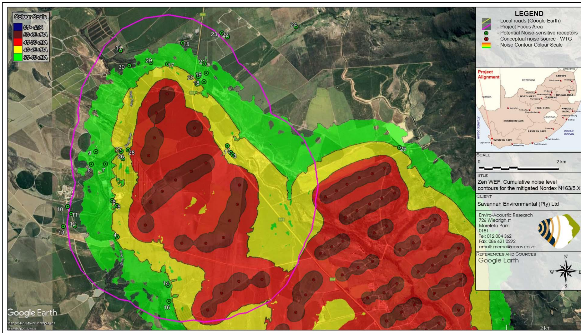
Figure 9-8: Projected future cumulative noise rating level contours (SPL of 107.2 dBA re 1 pW for the mitigated Nordex)
