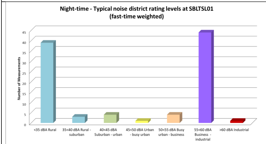
Figure 4-7: Classification of night-time measurements in typical noise districts at SBLTSL01
