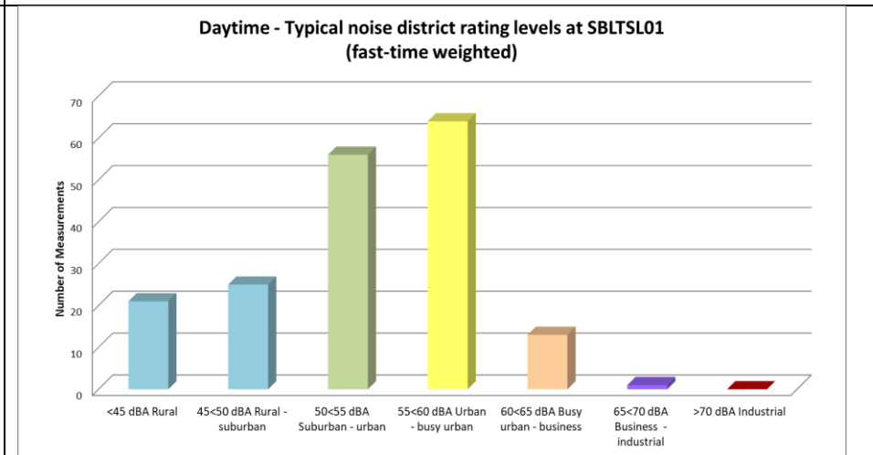
Figure 4-8: Classification of daytime measurements in typical noise districts at SBLTSL01
