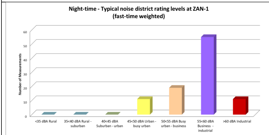
Figure 4-15: Classification of night-time measurements in typical noise districts at ZAN-1
