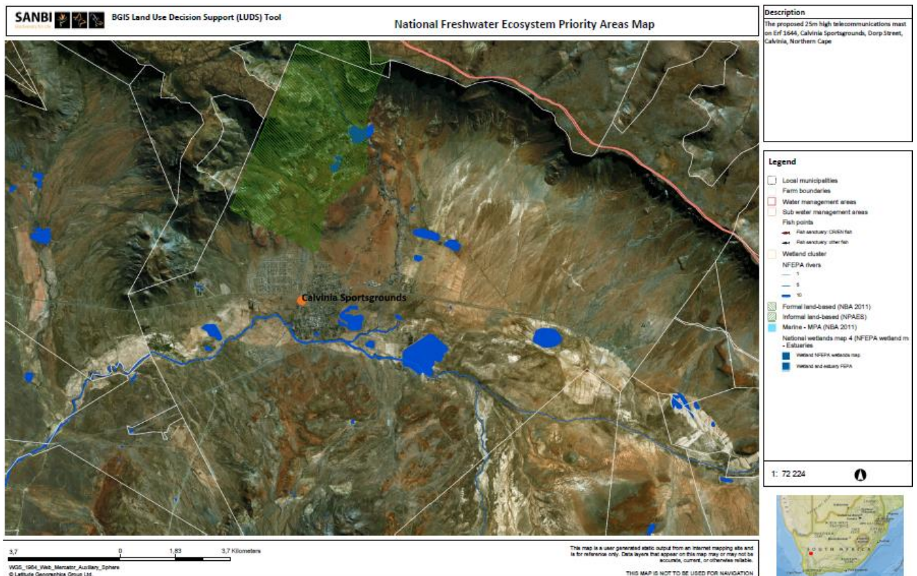
Figure 4: National Freshwater Ecosystem Priority Areas (NFEPA) Map of the proposed site (orange dot) and surroundings.
