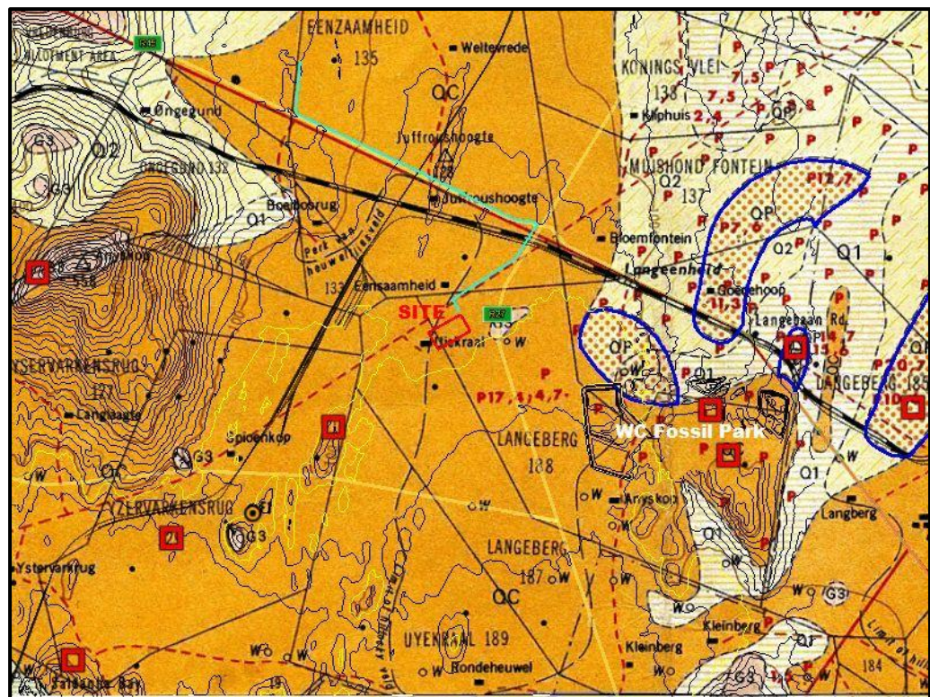
Figure 4. . Geology of the surrounding area. Extract from Visser & Schoch (1972), 1:125000 Map Sheet 255: 3217D & 3218C (St Helenabaai), 3317B & 3318A (Saldanhaabai). Viewed in Google Earth with 5 m contour overlay. The 25 m asl. contour is highlighted in yellow.
