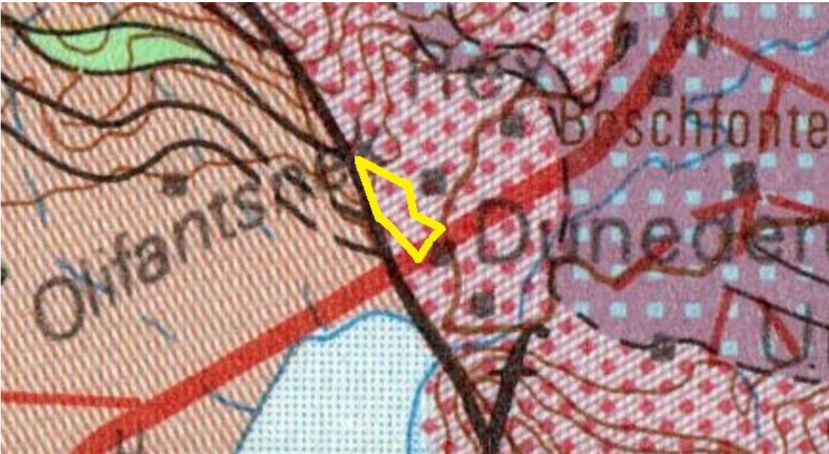
Figure 2: Geological map of study site (yellow polygon) and surroundings (adapted from the Rustenburg 2526 1:250 000 Geology Map)
