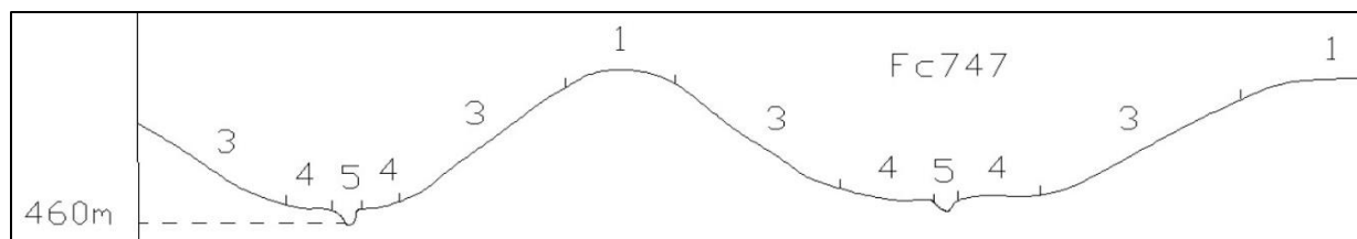
Figure 8-6 Illustration of land type Fc 747 terrain unit (Land Type Survey Staff, 1972 - 2006)
