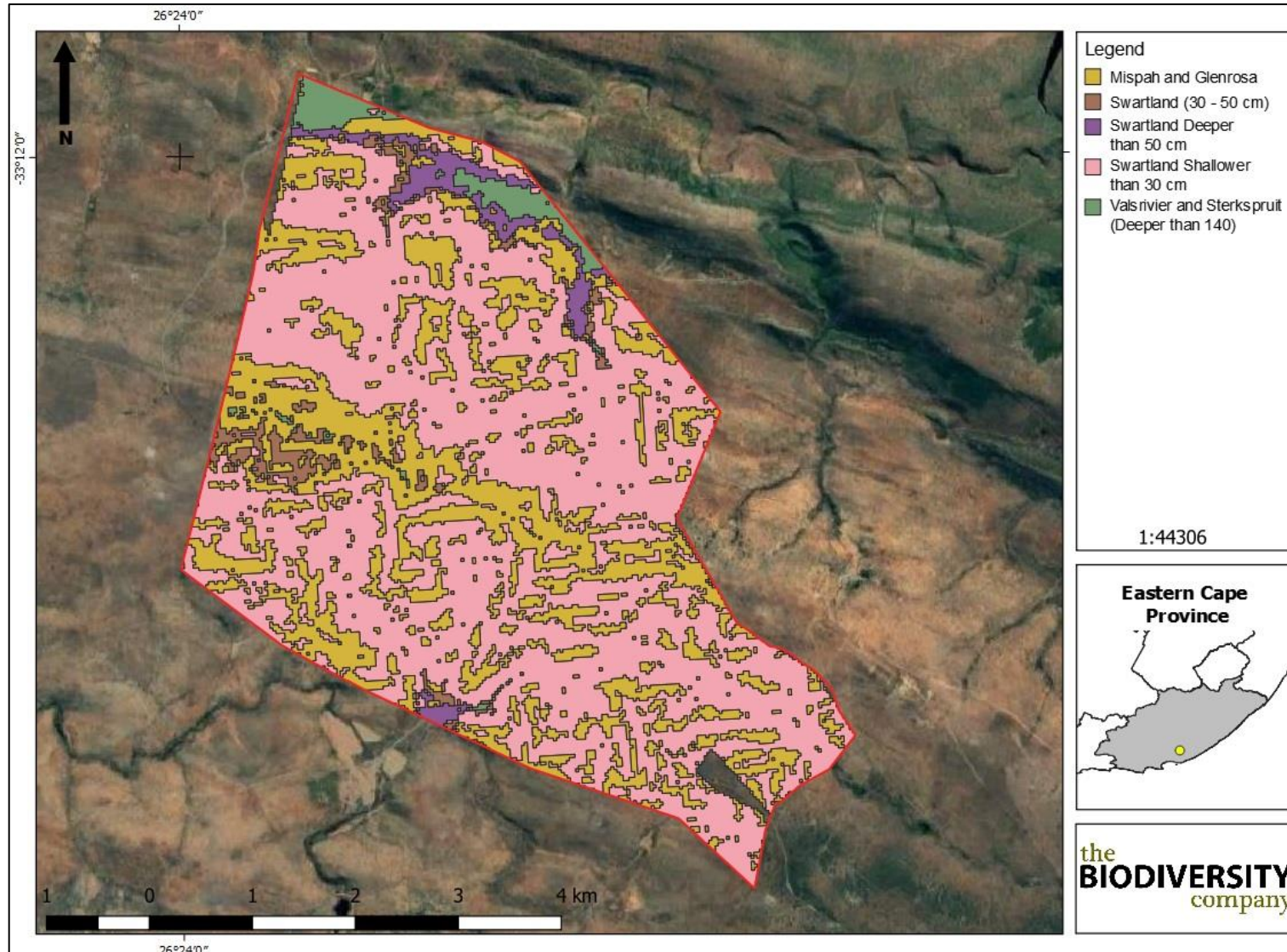
Figure 9-1 Soil delineations within the project area
