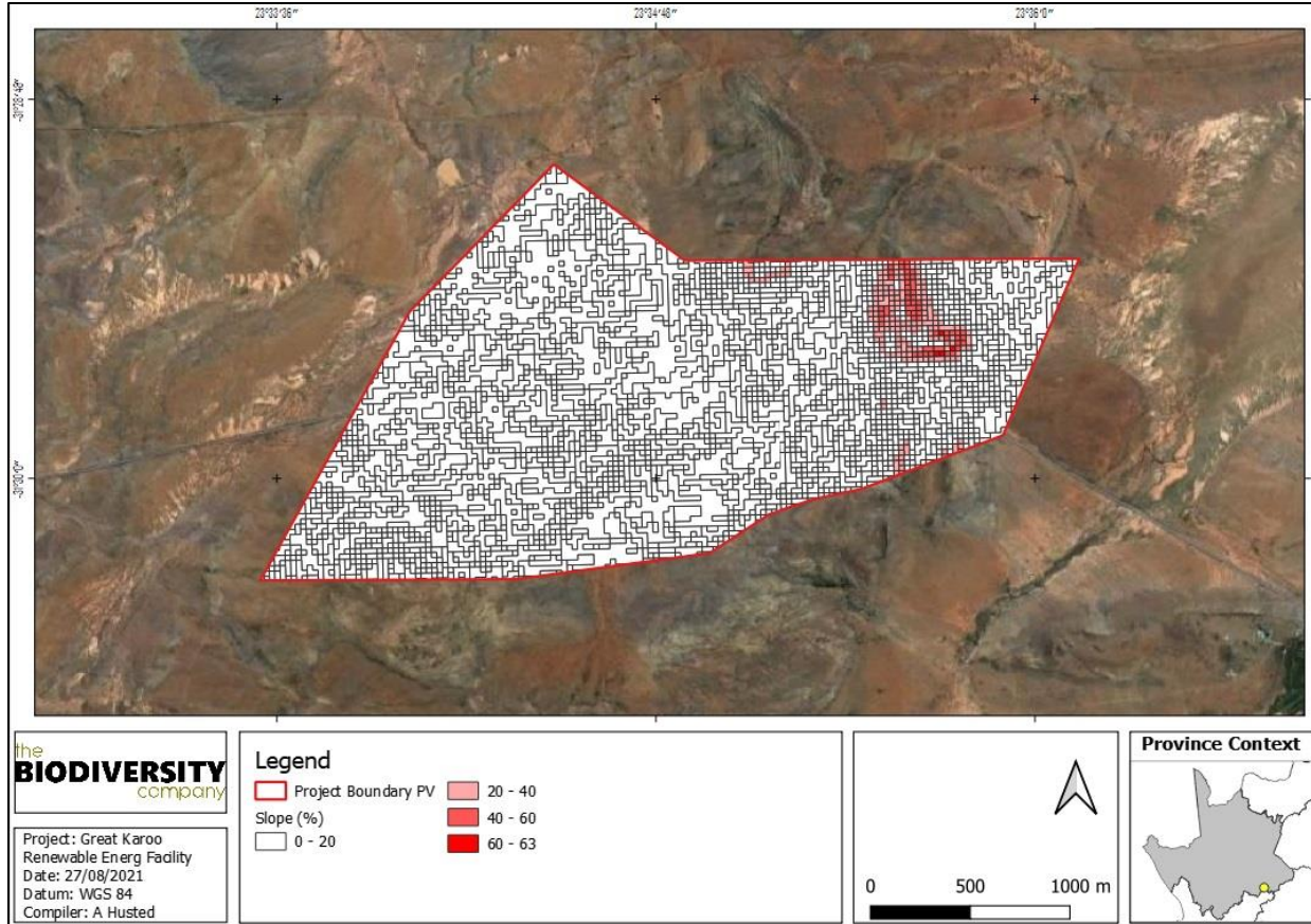
Figure 7-5 The slope percentage calculated for the project area
