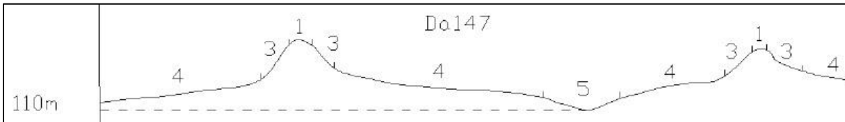
Figure 7-3 Illustration of land type Da 147 terrain unit (Land Type Survey Staff, 1972 - 2006)
