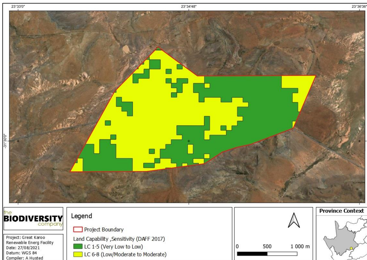
Figure 8-2 Land Capability Sensitivity (DAFF, 2017)
