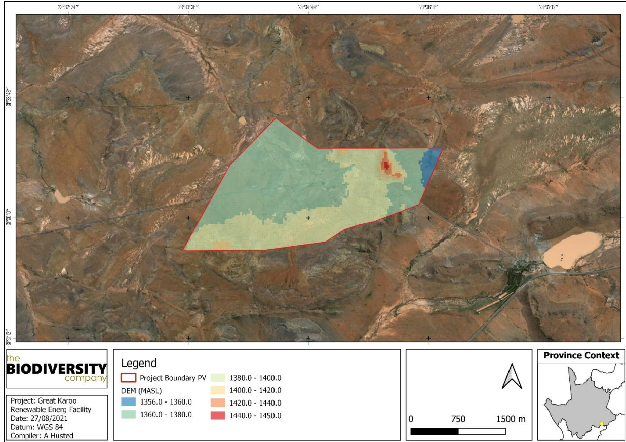
Figure 7-6 The DEM generated for the project area
