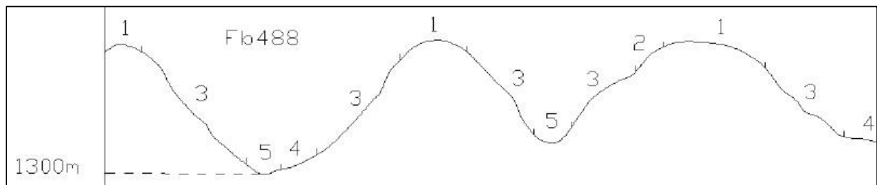
Figure 7-4 Illustration of land type Fb 488 terrain unit (Land Type Survey Staff, 1972 - 2006)
