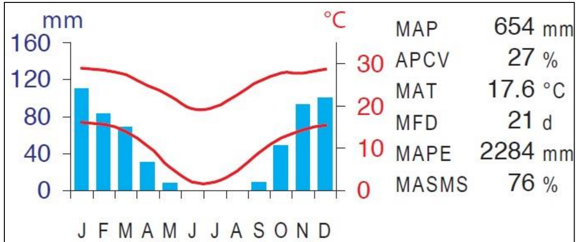
Figure 7-1 Climate for the region
