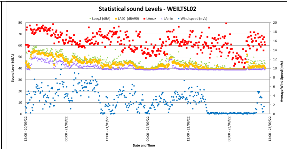
Figure 4-9: Maximum, minimum and statistical values at WEILTSLO2
