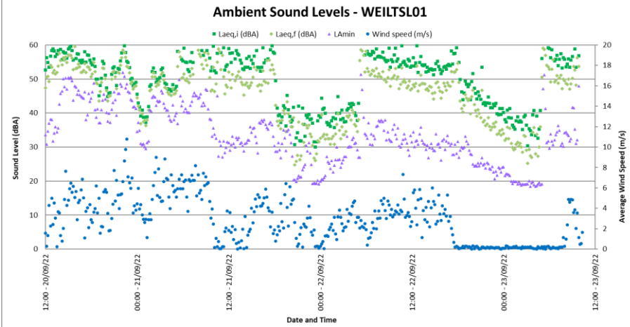
Figure 4-4: Ambient Sound Levels at WEILTSLO1
