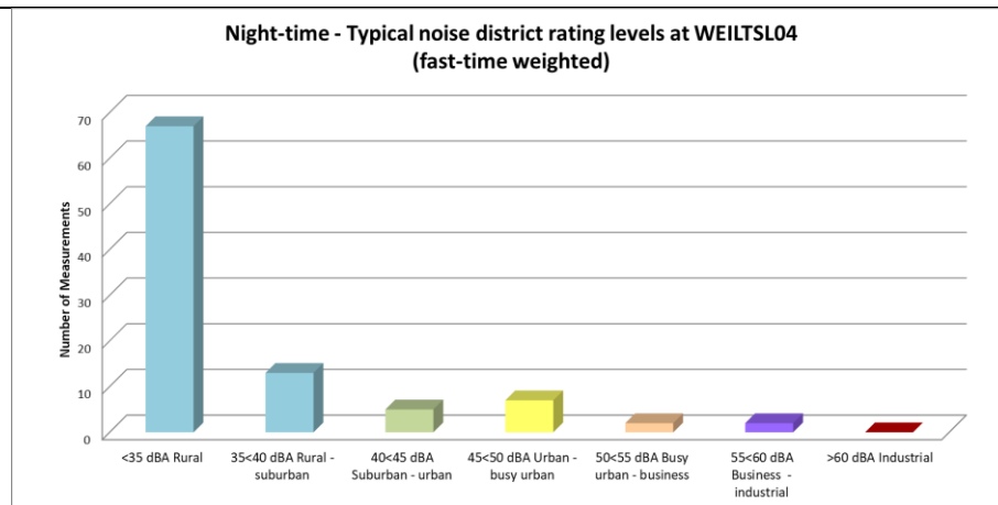
Figure 4-18: Classification of night-time measurements in typical noise districts at WEILTSL04
