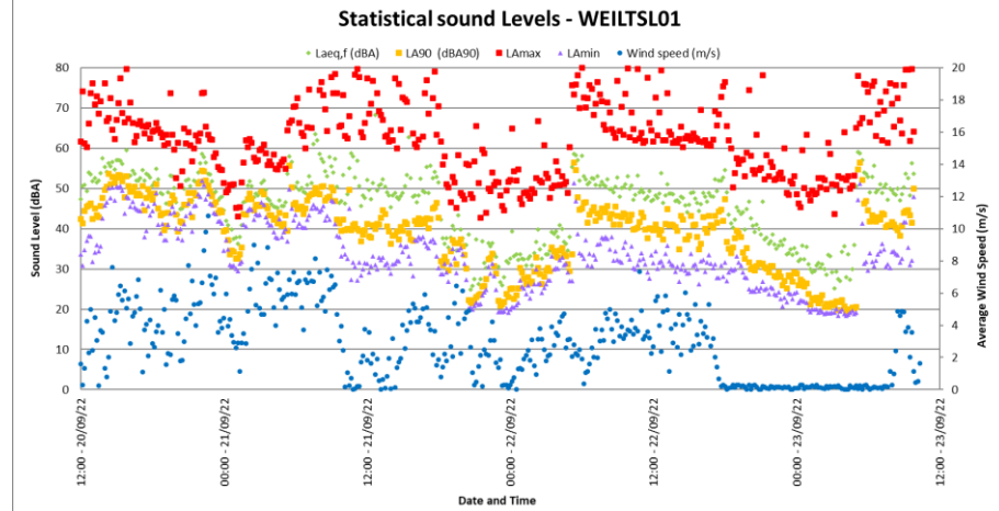
Figure 4-5: Maximum, minimum and Statistical sound levels at WEILTSLO1
