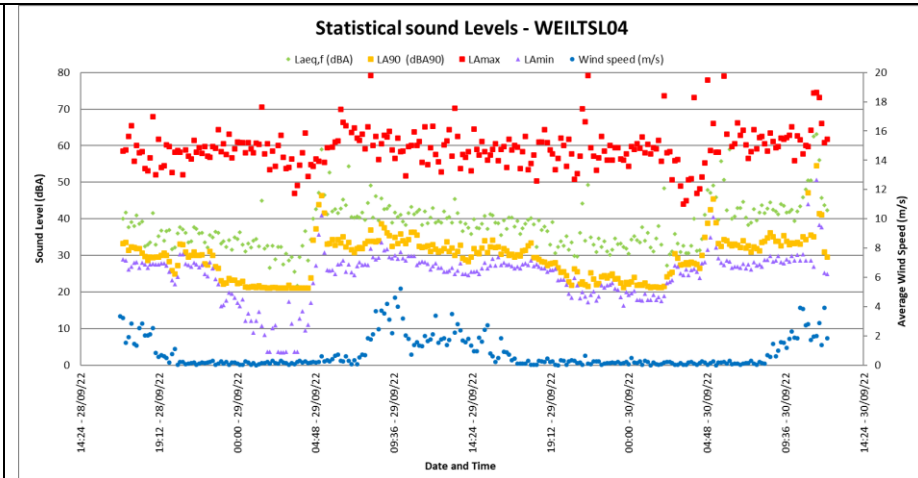
Figure 4-17: Maximum, minimum and Statistical sound levels at WEILTSL04
