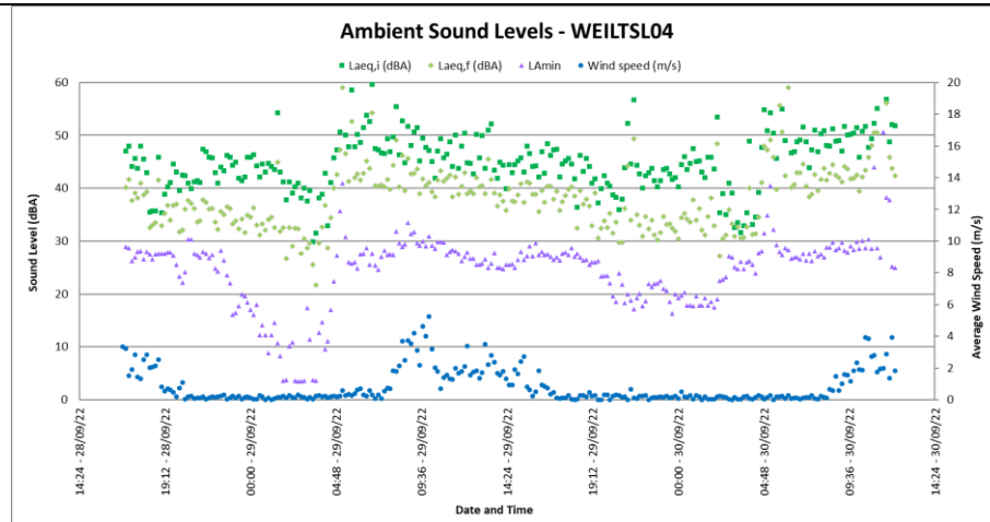
Figure 4-16: Ambient Sound Levels at WEILTSL04
