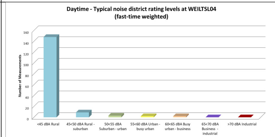
Figure 4-19: Classification of daytime measurements in typical noise districts at WEILTSL04
