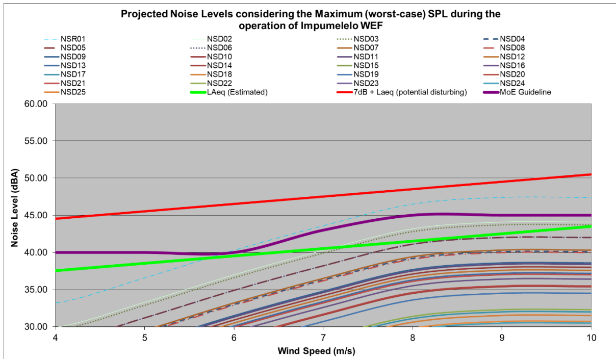
Figure 10-1: Projected noise levels at different wind speeds considering a WTG with worst-case SPL (noise levels exceeding potential ambient sound levels)
