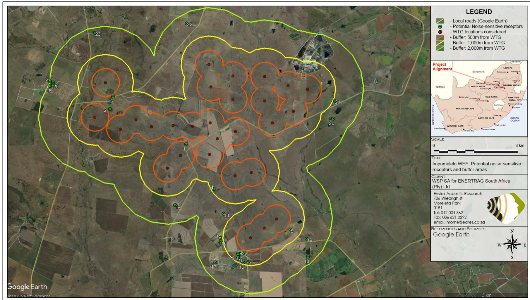
Figure 2-3: Study area and potential noise-sensitive receptors close to the Impumelelo WEF
