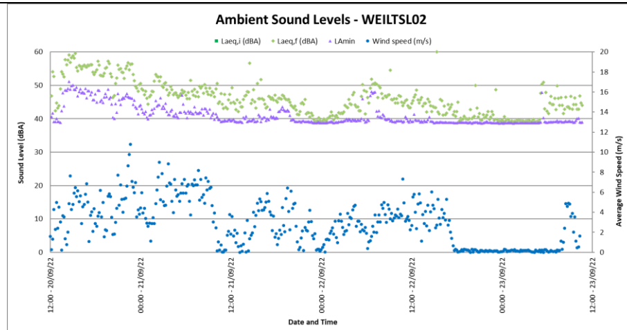
Figure 4-8: Ambient sound levels at WEILTSLO2
