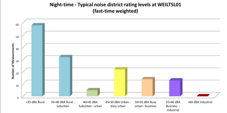
Figure 4-6: Classification of night-time measurements in typical noise districts at WEILTSLO1
