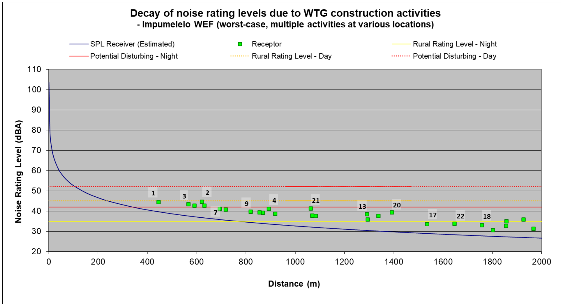
Figure 9-2: Projected conceptual construction noise levels – Impumelelo WEF
