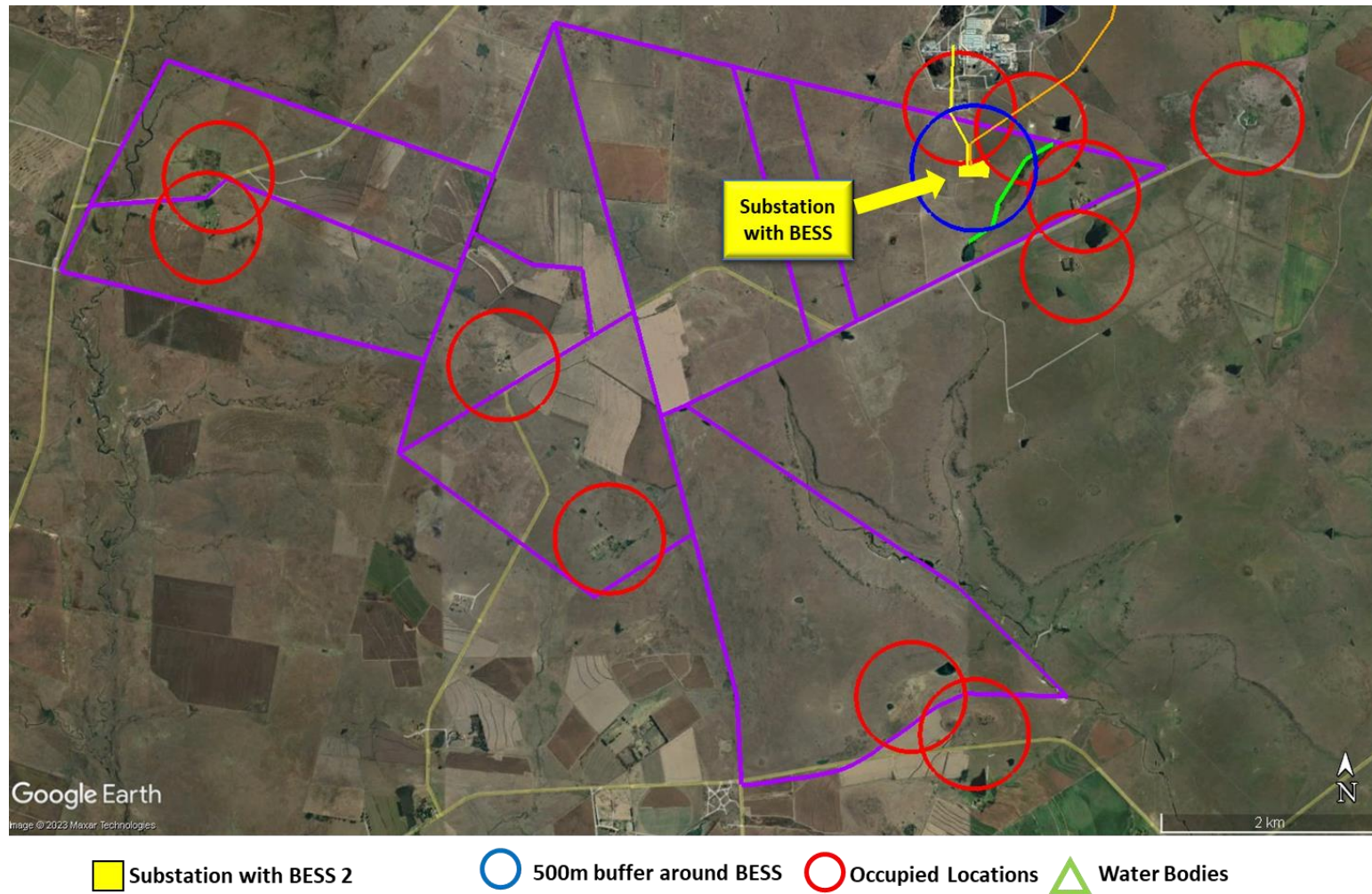
Figure 2.1.3 – 500m circles around the BESS Facilities (Blue) and Location of Farmhouses/Mines (Red) and Nearby Water Courses/Bodies (Green) in the immediate area
