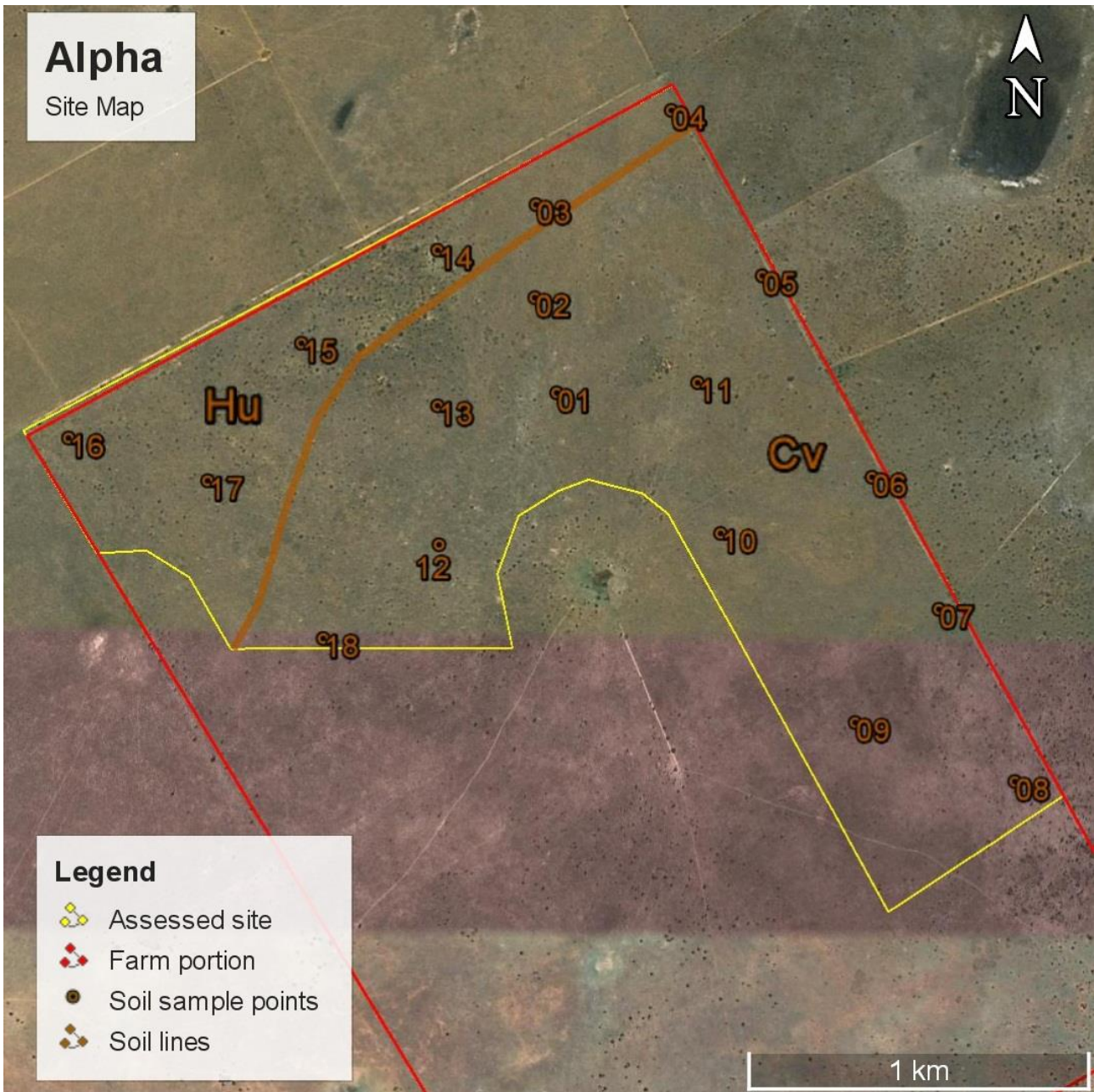
Figure 3. Satellite image of the assessed site (285 hectares) with soil information including identified soil form labels. Soil sample numbers correspond to those in Table A2. The surface coverage of each soil form is given in Table A3.
