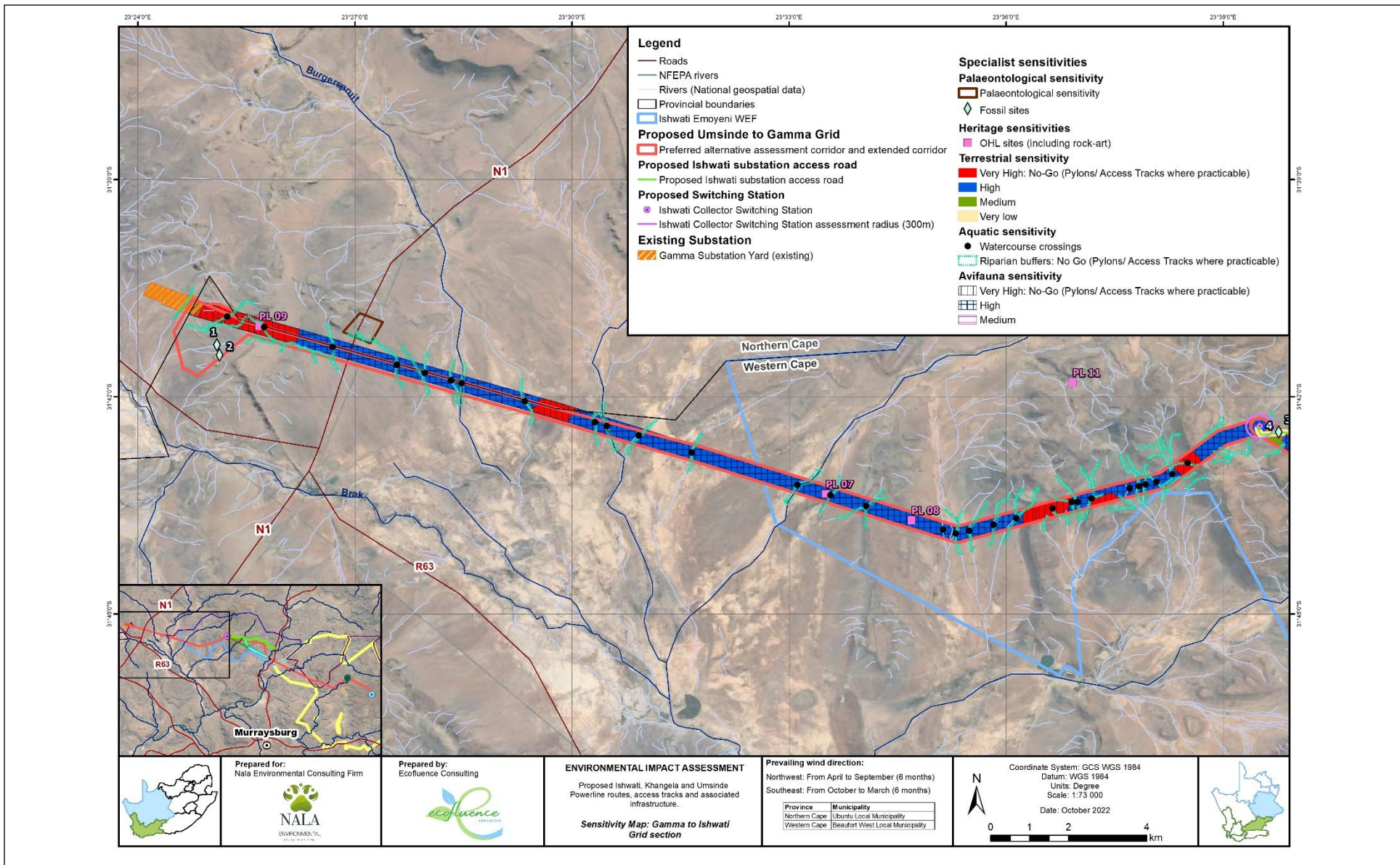
Figure 7: Sensitivity map of the proposed new 132kV powerline within the 400m corridor associated with the authorised Emoyeni Wind Energy Facilities from the Gamma MTS to the Ishwati Switching Station
