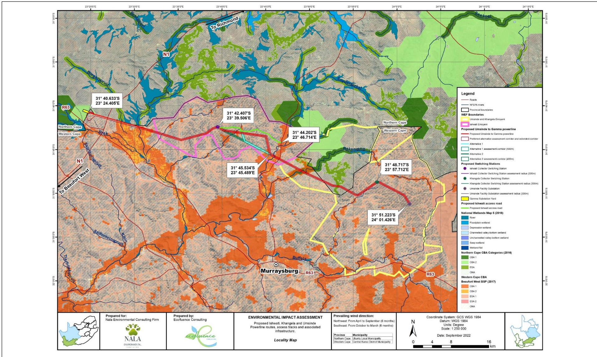
Figure 2: Locality Map of the proposed new 132kV powerline within the 400m corridor associated with the authorised Emoyeni Wind Energy Facilities
