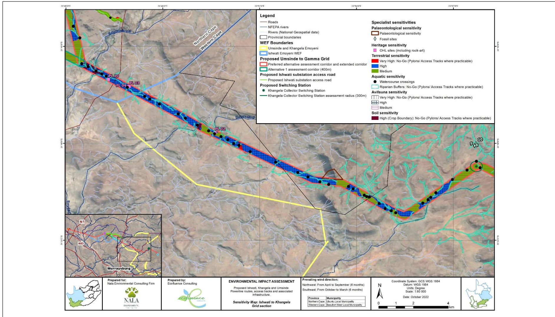
Figure 5: Sensitivity map of the proposed new 132kV powerline within the 400m corridor associated with the authorised Emoyeni Wind Energy Facilities from the Ishwati switching station to the Khangela Switching Station
