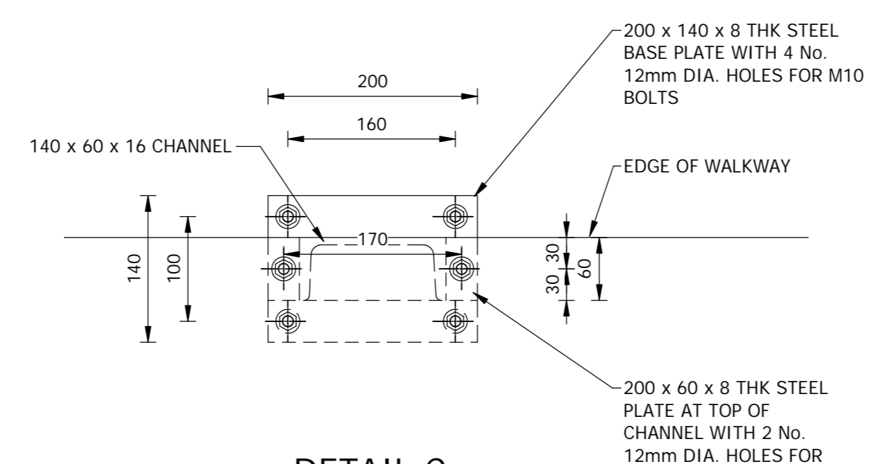
DETAIL C 1:5
