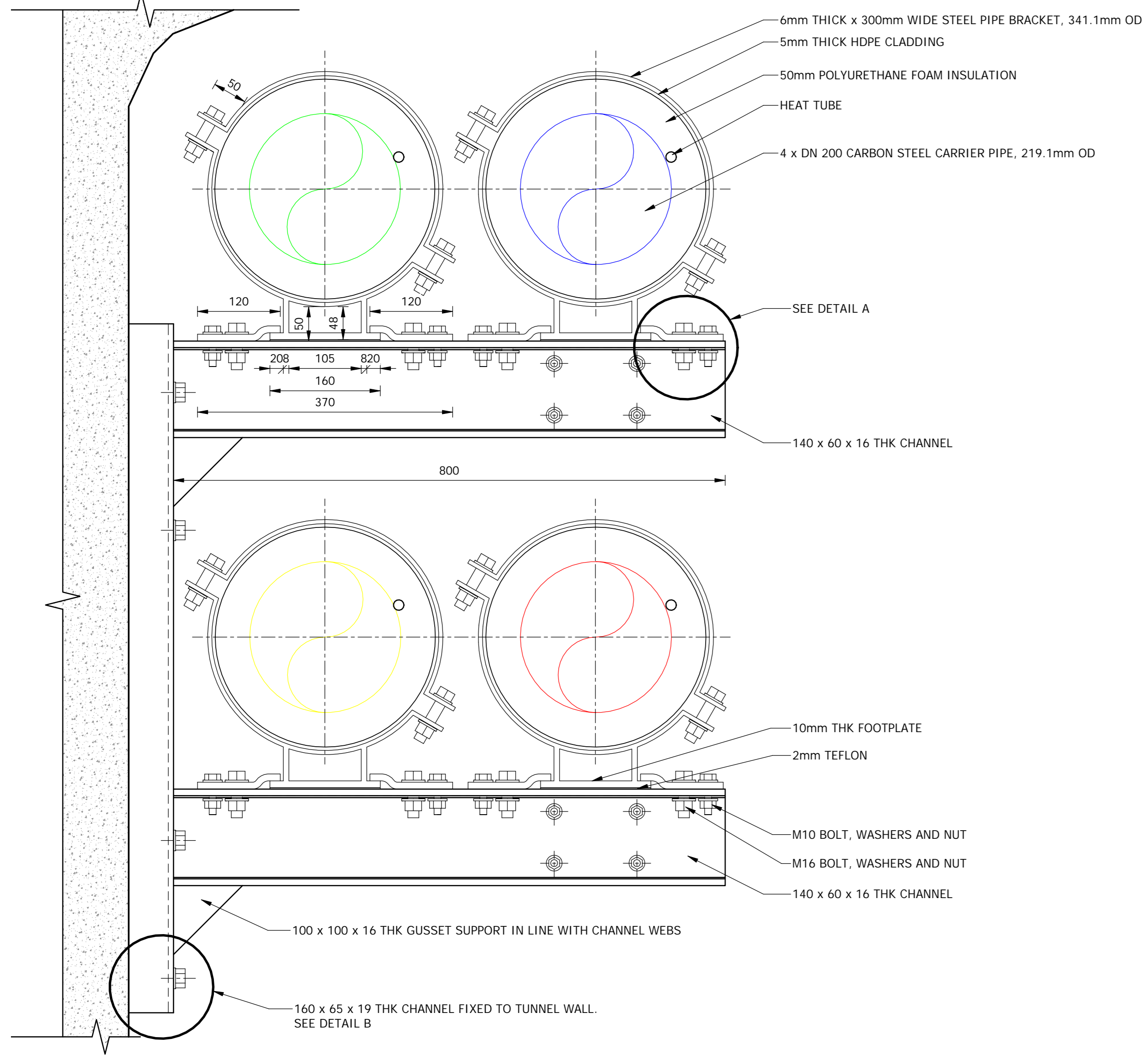
FRONT VIEW 1:5
