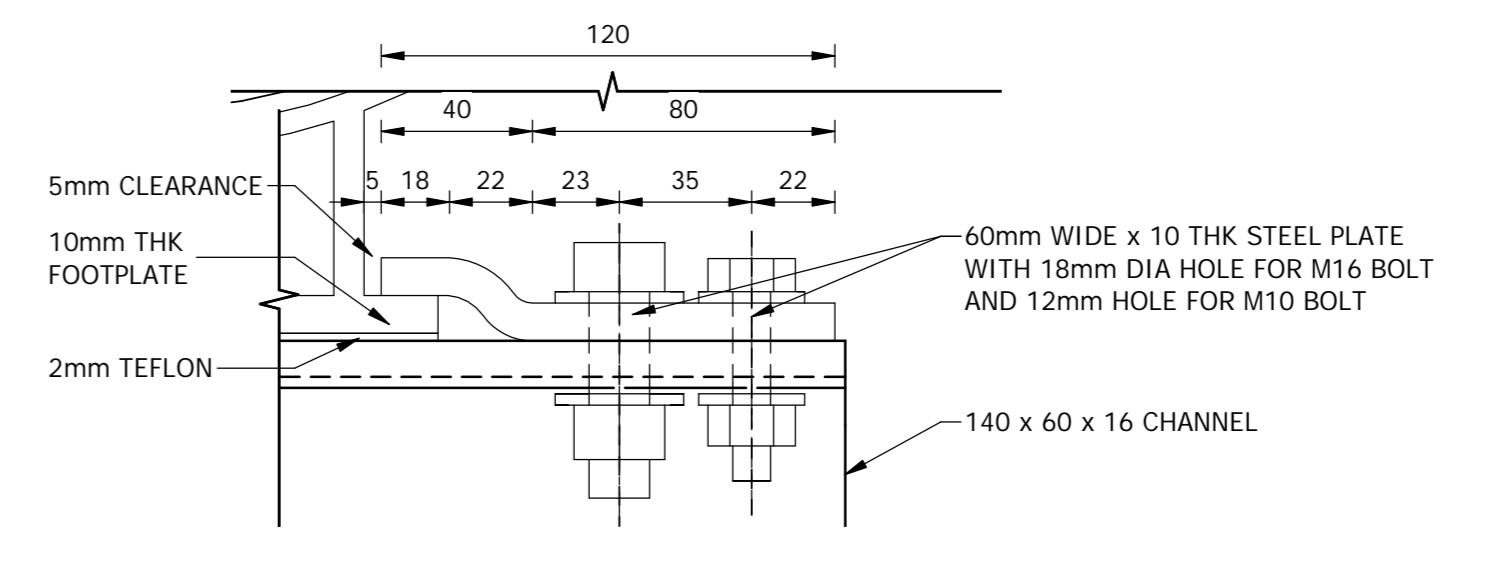
DETAIL A 1:2
