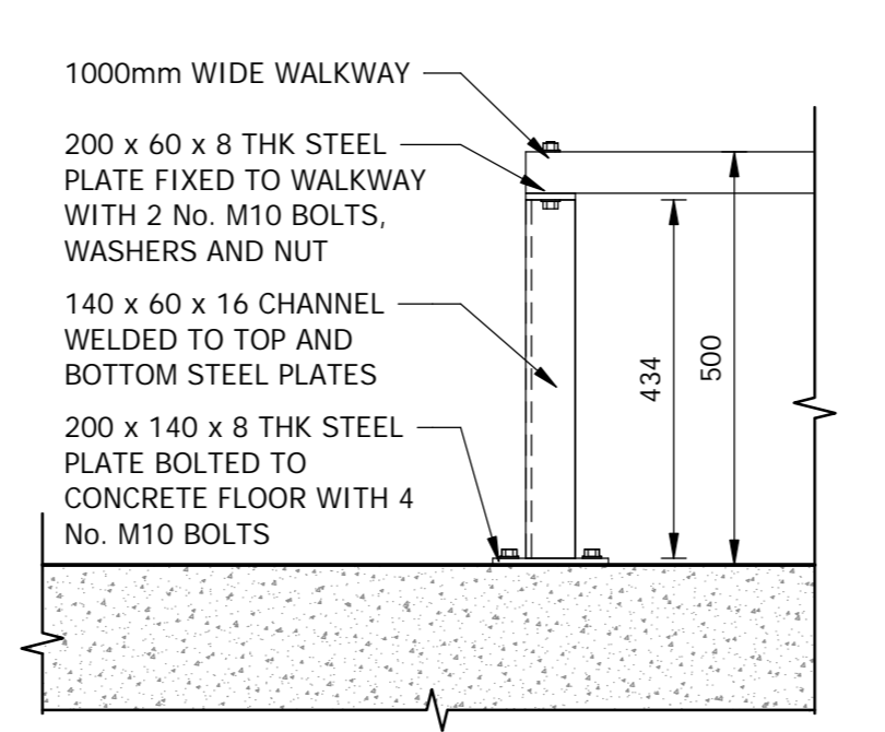
WALKWAY FIXING DETAILS (SEE DETAIL C) 1:10
