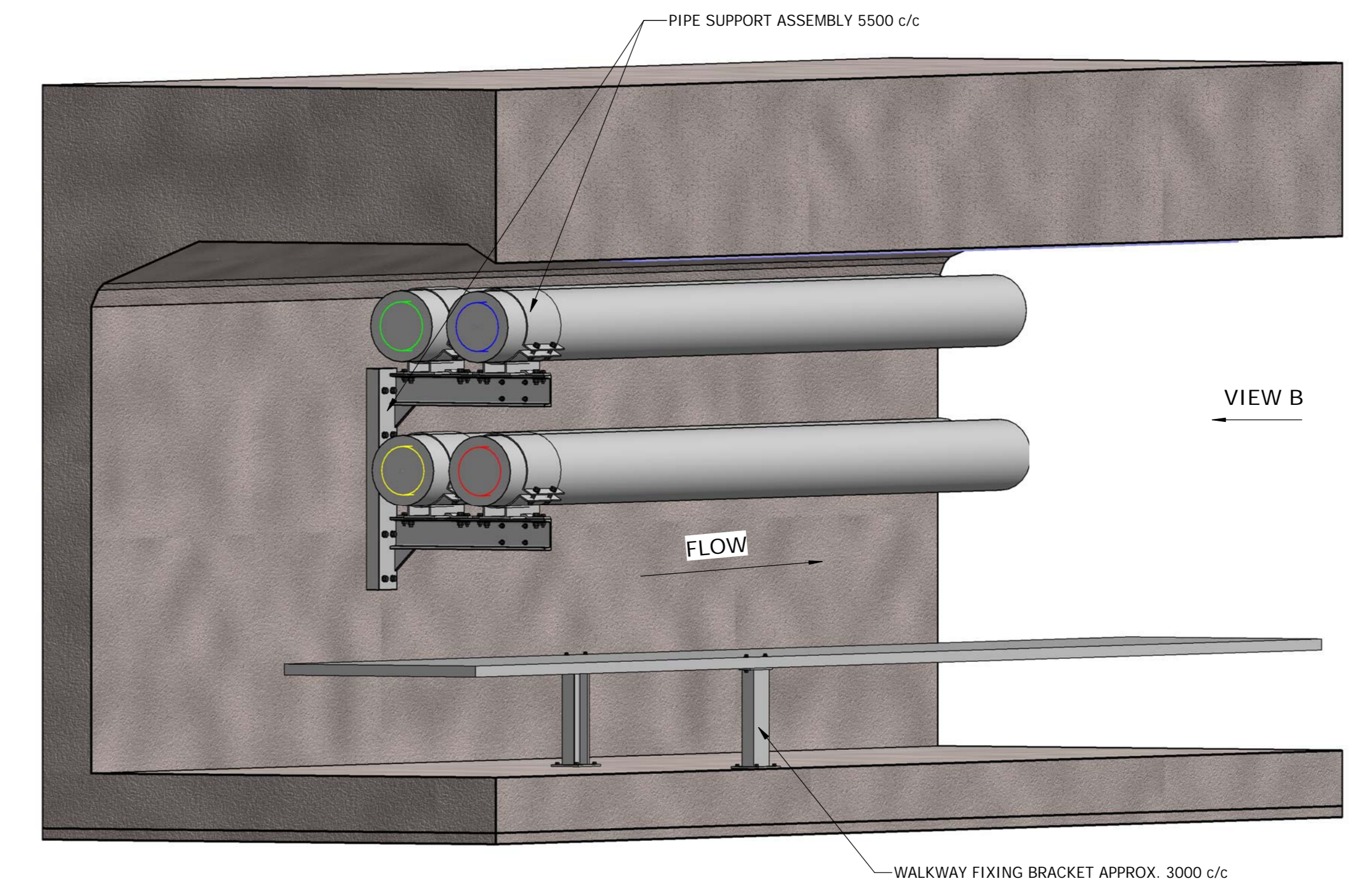
3D VIEW B
