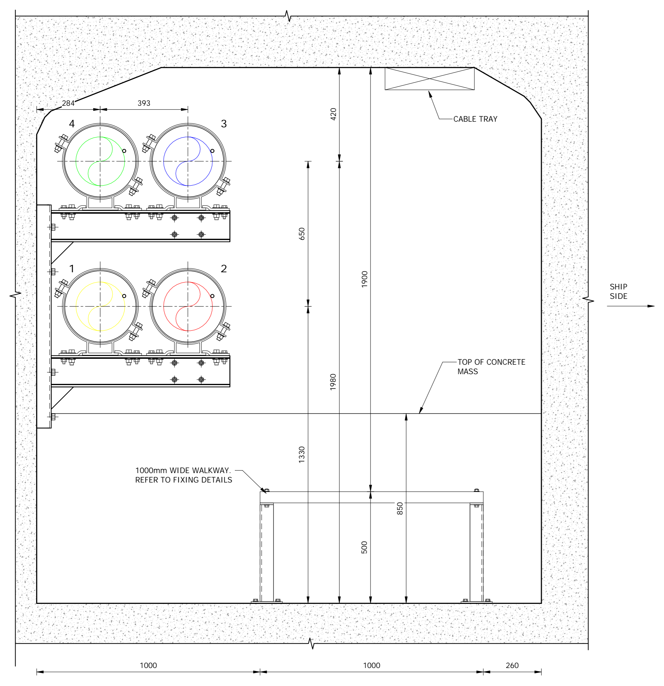
TYPICAL SECTION THROUGH TUNNEL 1:10
