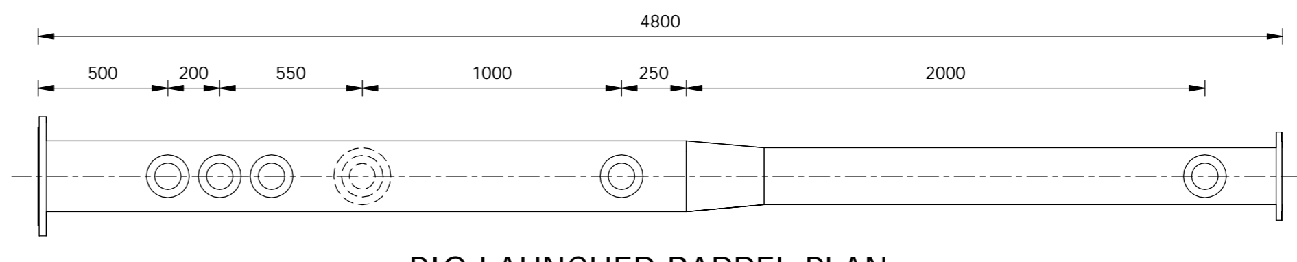
PIG LAUNCHER BARREL PLAN 1 : 20
