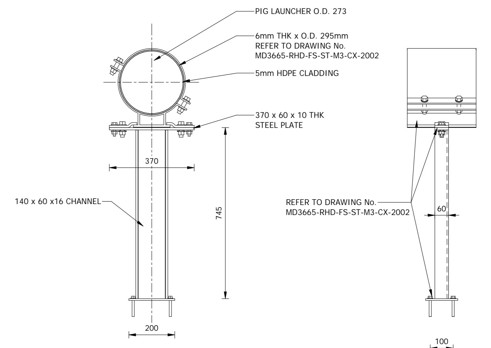
FRONT VIEW 1 : 10
