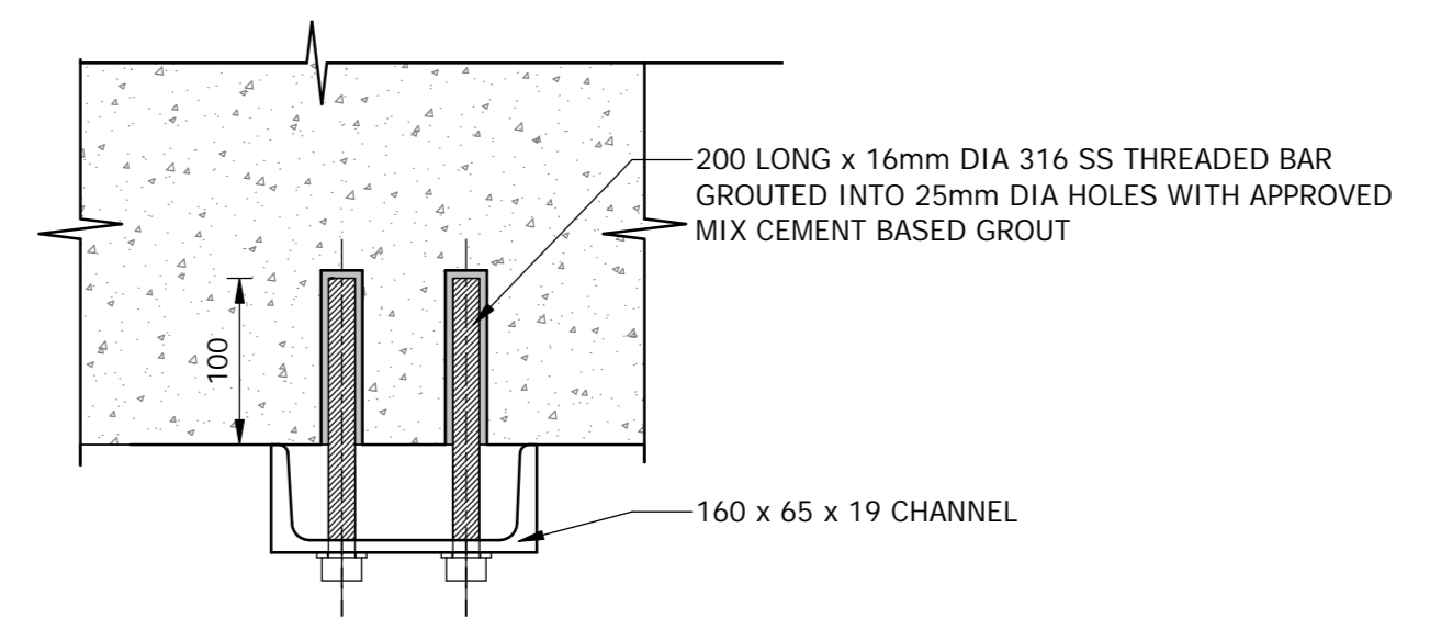
DETAIL B 1:5
