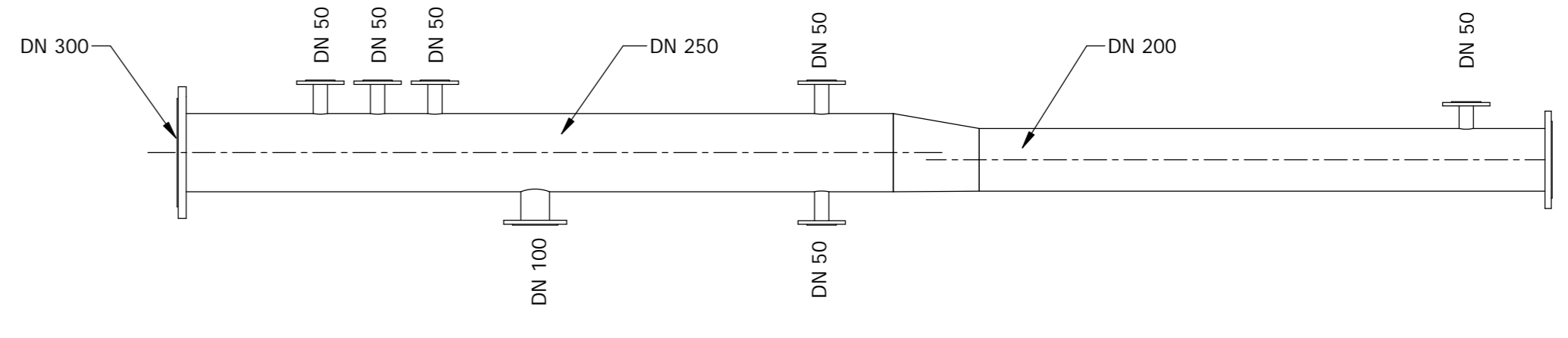
TYPICAL ELEVATION OF PIG BARREL 1 : 20
