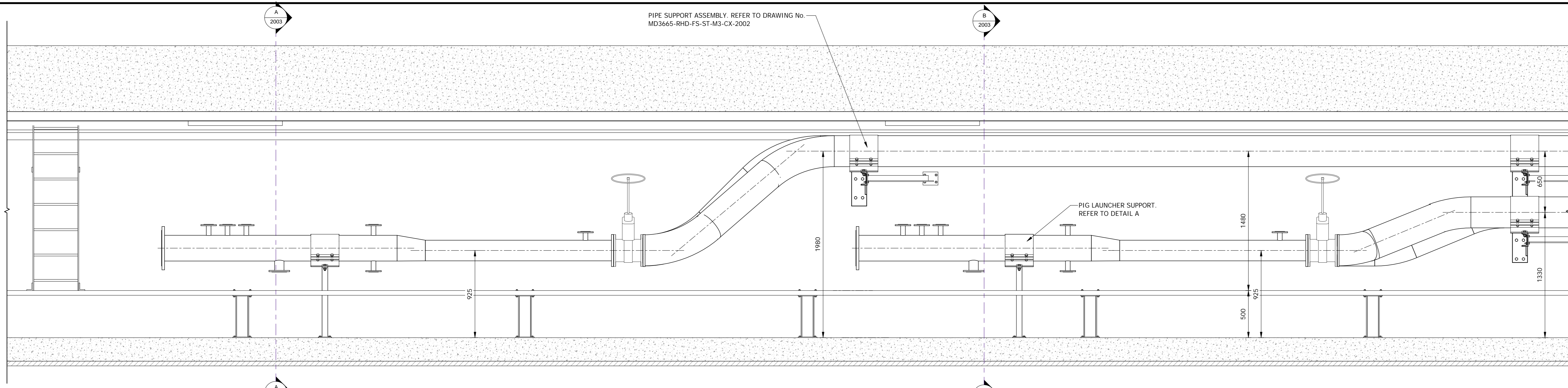
TYPICAL ELEVATION OF PIG LAUNCHER 1 : 20
