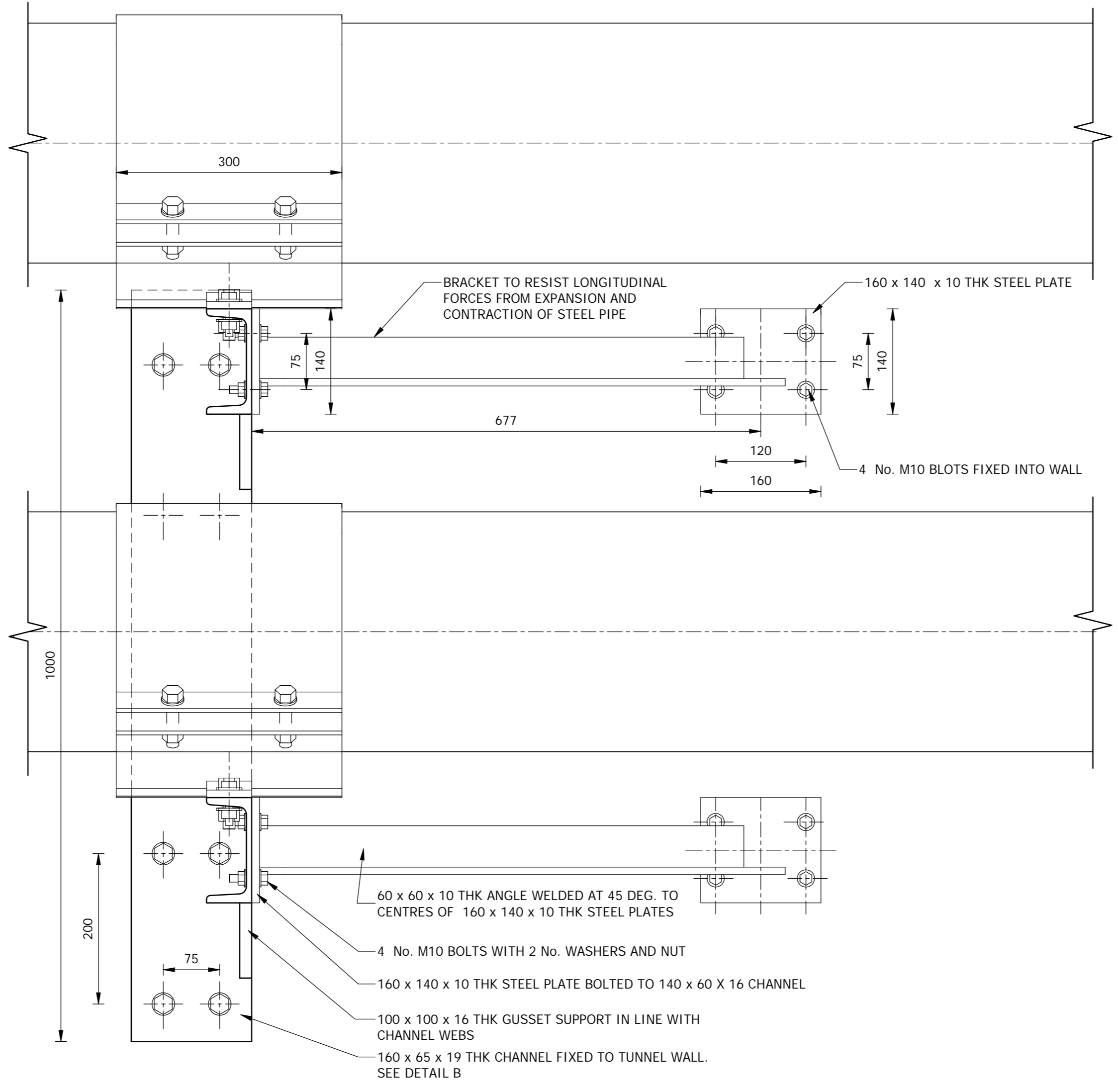
SIDE VIEW 1:5
